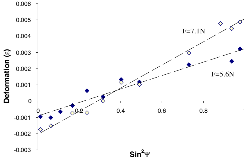
Fig. 3. \ln(1/\sin\theta_{101})-\sin^2\Psi values calculated for the 1 0 1 peak by the application of the DRAST method [13] for two applied load states.
