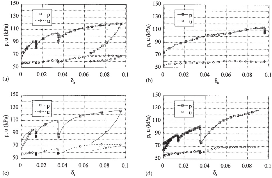
Figure 25. Pressure and pore water pressure at the cavity wall during pressio triax tests. (a) Test TA ( \delta_a = 3 \times 10^{-5} \text{ s}^{-1} ; 50 \text{ mm}^3/\text{min} ); (b) test TB ( \delta_a = 6 \times 10^{-7} \text{ s}^{-1} ; 1 \text{ mm}^3/\text{min} ); (c) test TC ( \delta_a = 1.5 \times 10^{-4} \text{ s}^{-1} ; 250 \text{ mm}^3/\text{min} ); (d) test TD ( \delta_a = 6 \times 10^{-6} \text{ s}^{-1} ; 10 \text{ mm}^3/\text{min} ).
