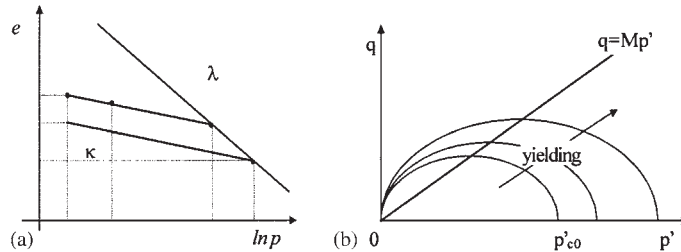
Figure 2. Modified Cam Clay model representation.
