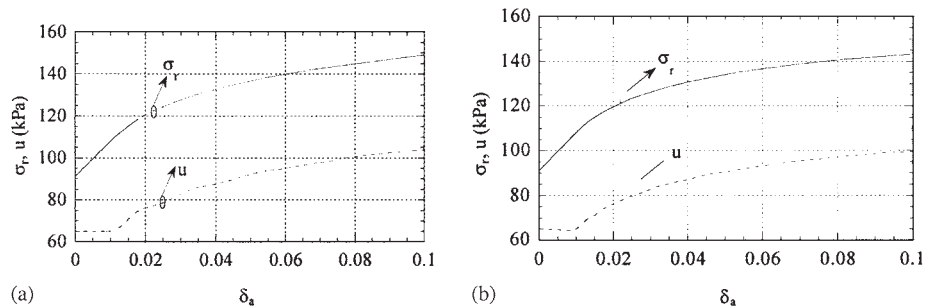
Figure 3. Numerical simulation of (a) pressuremeter test; (b) and pressio triax test.
