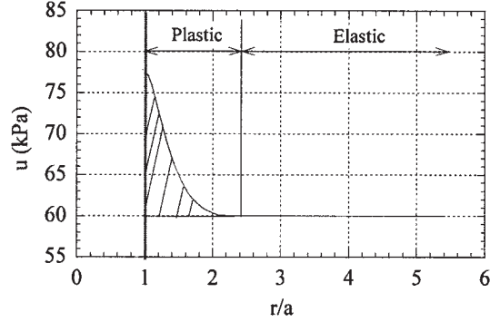
Figure 18. Pore pressure dissipation during strain holding test.
