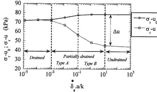
Figure 12. Evolution of the total stress \sigma_r - u_0 and of effective stress \sigma_r - u as a function of the variable \delta_a/ka .
