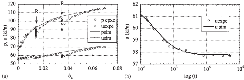
Figure 27. Comparison between experiment and simulation of test TA.
