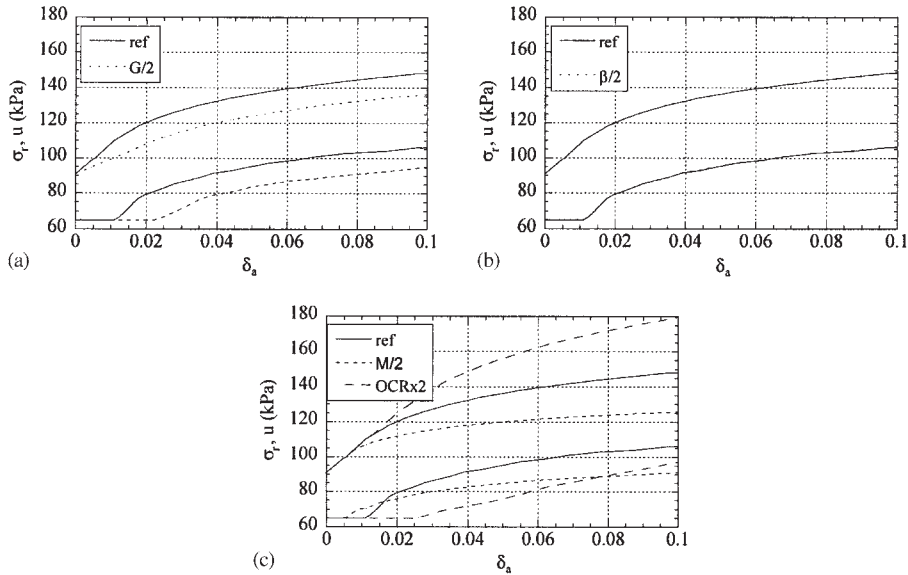
Figure 22. Modified Cam Clay parameter effects on the pressuremeter curve. (a) G effects; (b) \beta effects; (c) M and p'_{c0} effects.
