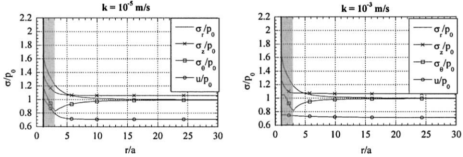
Figure 7. Stress distribution along a radius for an applied pressure of 60 kPa for different permeability.
