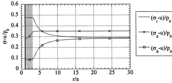
Figure 5. Effective stress distributions for \delta_a = 10\% .
