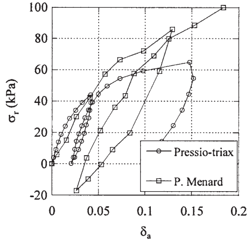
Figure 24. Comparison between pressuremeter curves from Menard pressuremeter test and pressio triax test [12].
