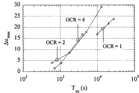
Figure 17. Effect of maximum excess pore pressure on time corresponding to 50% dissipation during strain holding test.
