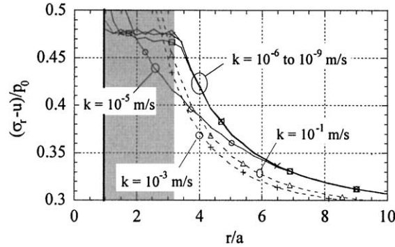
Figure 8. Variation of effective stress (\sigma_r - u)/p_0 along a radius for soil permeability varying from 10^{-1} to 10^{-9} m/s.
