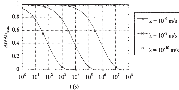
Figure 14. Permeability effect on pore pressure dissipation curves (OCR = 2, \delta_a = 4\% ).
