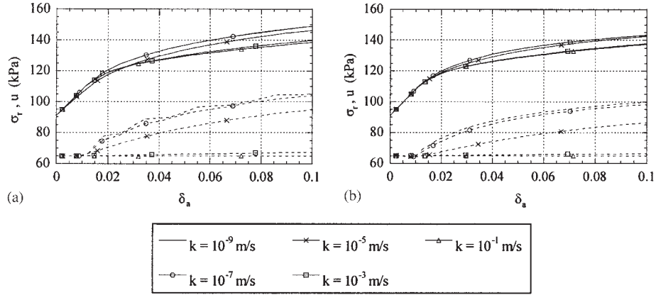
Figure 6. Permeability effect on stress strain curves for pressuremeter tests (a) and pressio triax tests (b).
