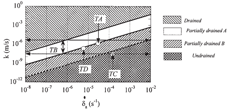
Figure 28. Drainage conditions during a pressio triax test regarding the permeability and the strain rate.
