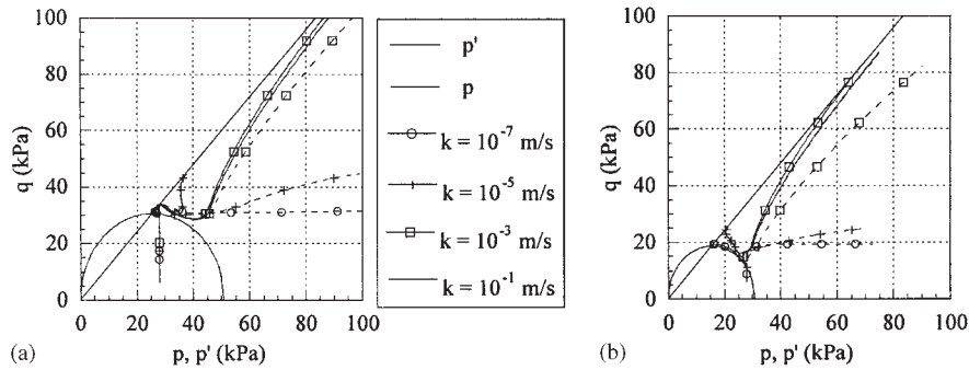
Figure 9. Permeability effect on pressuremeter stress path: (a) p'_{c0} = 51 kPa; (b) p'_{c0} = 31 kPa.
