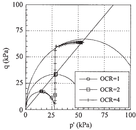
Figure 10. Stress paths obtained for overconsolidation ratio of 1, 2 and 4 for permeability equal to 1 \times 10^{-9} m/s.
