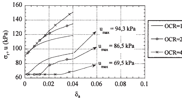
Figure 15. Effect of overconsolidation ratio on pressuremeter and pore pressure curve before strain holding test.
