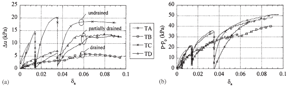
Figure 29. Excess pore water pressure generated during pressio triax tests.
