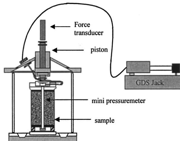
Figure 23. Pressio triax apparatus.
