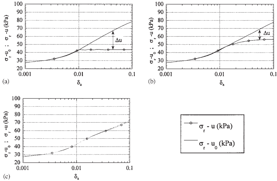
Figure 11. Pressuremeter curves in a p - \ln(\delta_a) diagram for different permeabilities. (a) k = 10^{-7} m/s; (b) k = 10^{-5} m/s; (c) k = 10^{-3} m/s.
