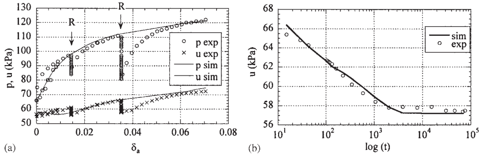
Figure 26. Comparison between experiment and simulation of test TC.
