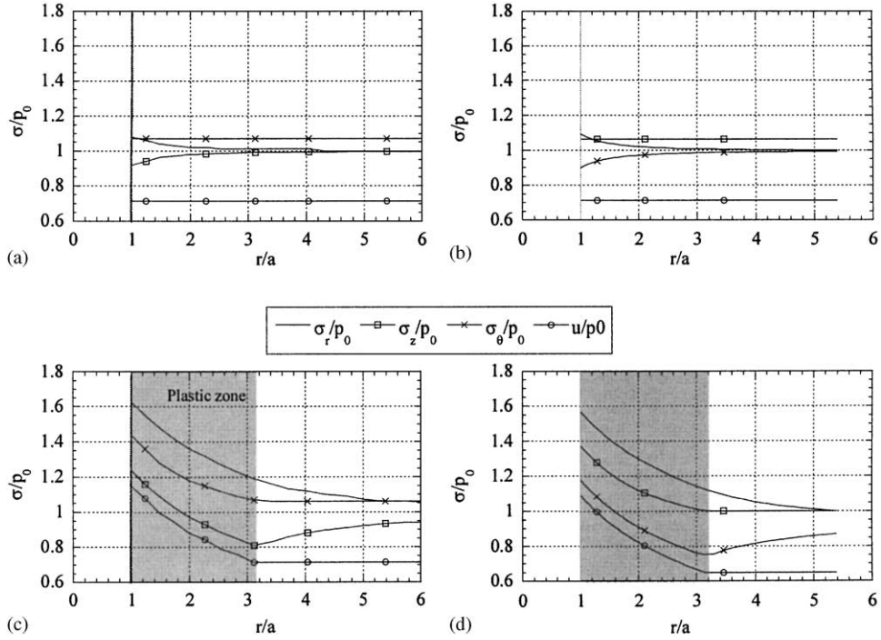
Figure 4. Stress distribution along the radius for \delta_a = 0.5\% for pressuremeter test (a) and pressio triax (b); for \delta_a = 10\% for pressuremeter test (c) and pressio triax (d).
