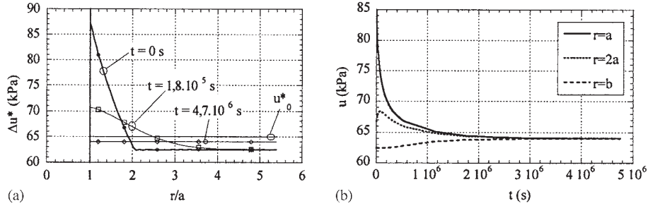
Figure 13. Pore water pressure distribution along a radius for different time (a); evolution with time for different (b).
