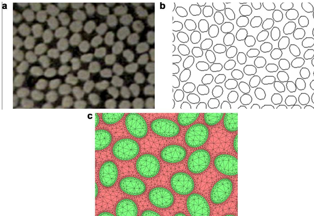
Fig. 4. Numerical model from a micrography: (a) micrography of a ply transverse section in a carbon fibre/ epoxy composite, (b) object analysis: elliptical sections of fibres, (c) mesh of the ply microstructure: fibres and matrix.
