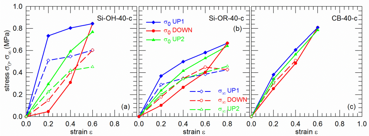
FIGURE 7 Evolution of the initial stress \sigma_0 and of the asymptotic limit \sigma_\infty determined by the power law equation (eq 4): (a) hydroxylated silica, (b) hydrophobic silica and, (c) carbon black fillers [the legend of the 3 figures is indicated in (b)]
