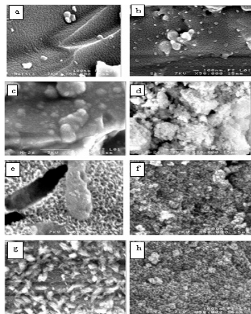
Figure 7: SEM micrographs; a, c, e and g for sample MB before and after immersion in SBF for 2,5, 7 days and b, d, f and h for sample SG-B before and after immersion in SBF for 2,5, 7 days, respectively.
