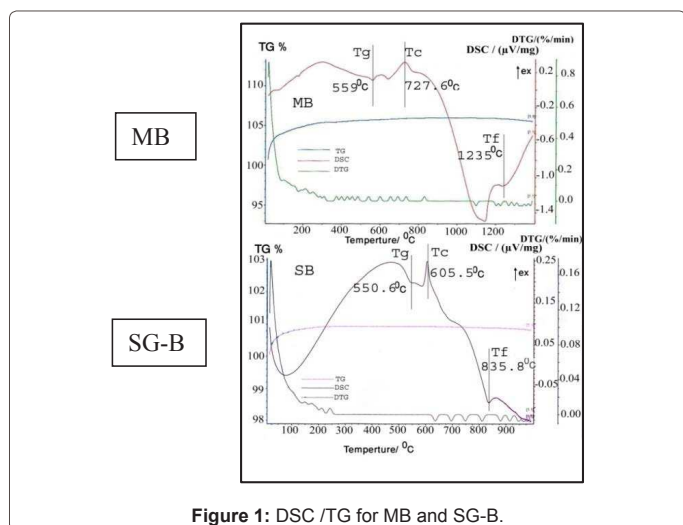
Figure 1: DSC /TG for MB and SG-B.
