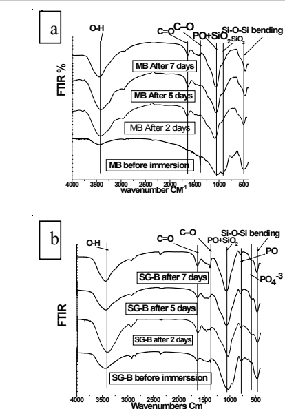
Figure 6: FTIR for samples a. MB and b. SG-B before and after immersion in SBF for 2, 5 and 7 days.
