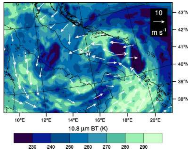
Figure 2. 10.8 \text{ m BT} (K, shading) and surface wind (vectors) obtained from MSG and QuikSCAT observations on 25 September 2006 at 1700 and 1654 UTC, respectively. The white star gives the position of the medicane as estimated by Moscatello et al. (2008a). This figure is available in colour online at wileyonlinelibrary.com/journal/qj
