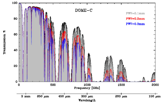
Fig. 1. Atmospheric transmission at 0.1, 0.2, and 0.3 mm PWV between 0–2 THz ( \approx 3 mm to \approx 150\ \mu\text{m} ) at Dome C calculated with the atmospheric model MOLIÈRE.
