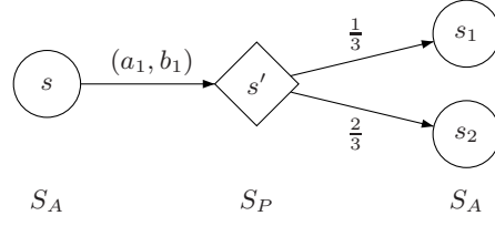
Fig. 3. Example of interaction separation for \delta(s, a_1, b_1)(s_1) = \frac{1}{3} and \delta(s, a_1, b_1)(s_2) = \frac{2}{3} .
