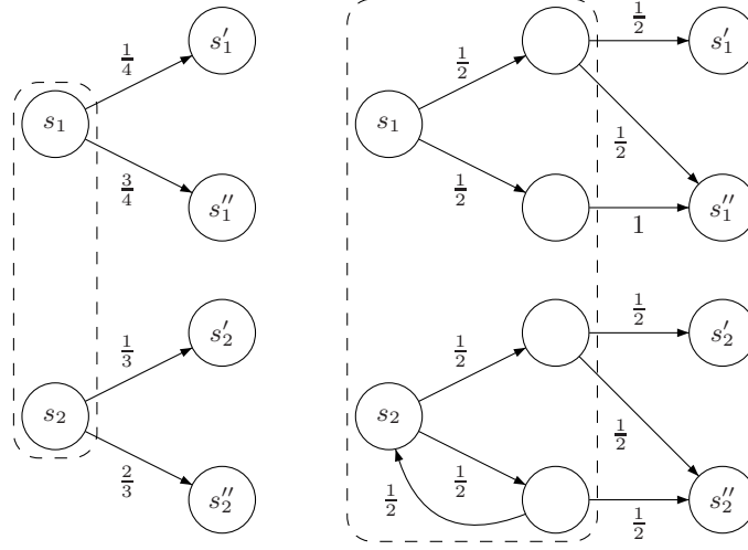
Fig. 4. An example showing why the uniform-binary reduction cannot be used with partial observation.
