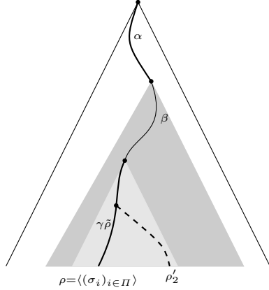
Fig. 11. Play \rho .
