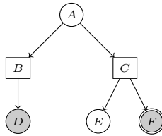
Fig. 2. Game \mathcal{G}' .
