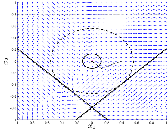
Figure 1. Phase space for the closed-loop system in Example 1 with |d|_\infty < 0.01 and a sampled-data implementation of the control with \bar{T} = 10^{-3} . Ellipsoid in dotted-dashed line – \Omega_0 . Ellipsoid in solid line – \Omega_\infty . Solid black lines – limiting hyperplanes of C_{(1-\rho)}\mathcal{V}(K) .
