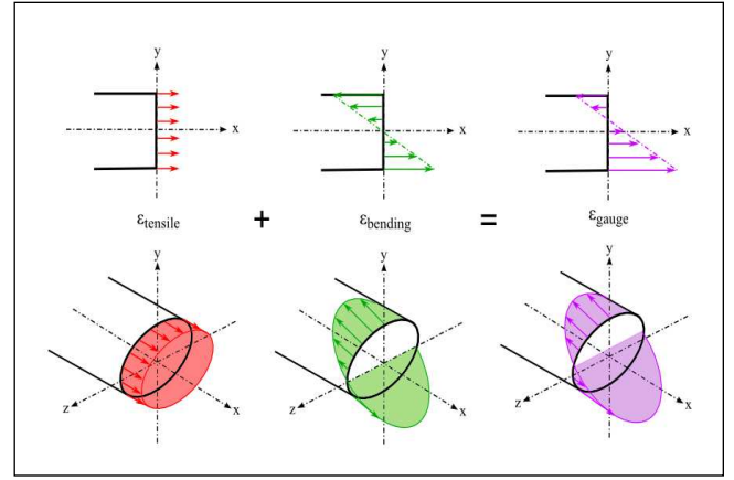
Figure 2. Superposition principle of a deformable needle.
