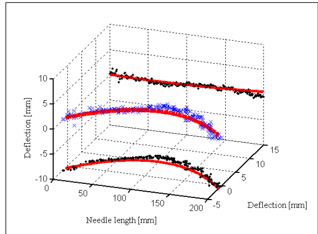
Figure 3. 3D reconstruction of a medical needle from two local strain measurements.
