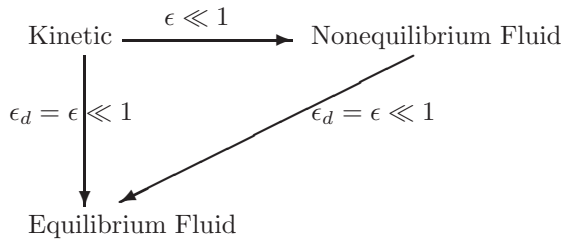
Figure 1: Schematic of the double Chapman-Enskog procedure
