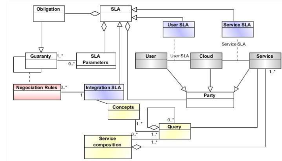
Figure 2. SLA extension
