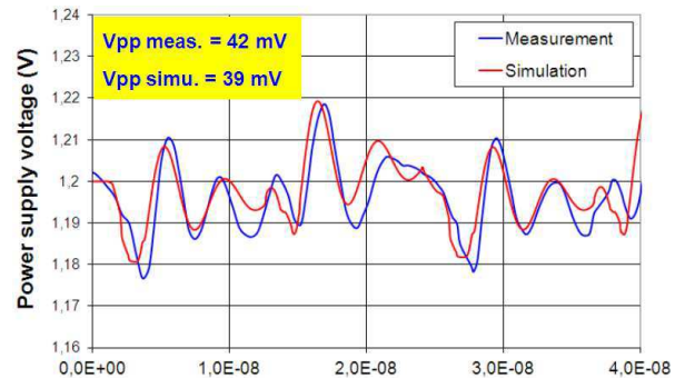
Fig. 7. Comparison between simulated power supply voltage bounce after 120 minutes of 3.6 V electrical stress
