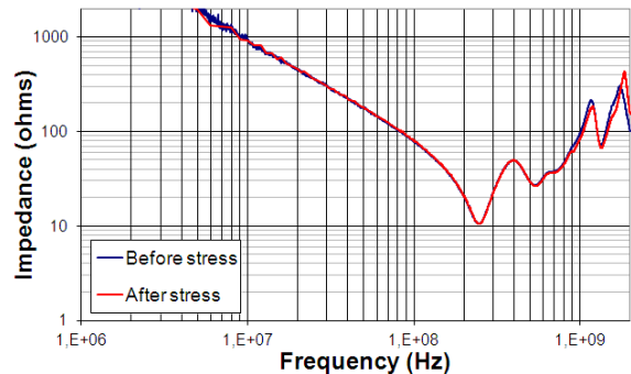
Fig. 3. Measurements of the impedance of the power distribution network of the digital core before and after electrical stress
