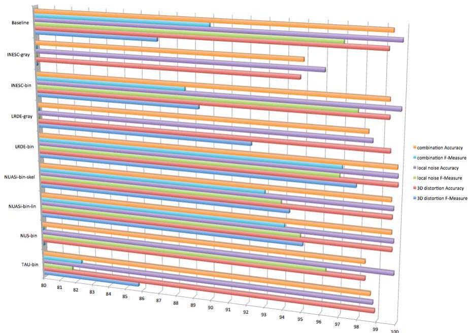
Fig. 7: Average music score competition results. The figure presents, for each participant method, the Average Accuracy and F-Measure of their method on the different sets.
