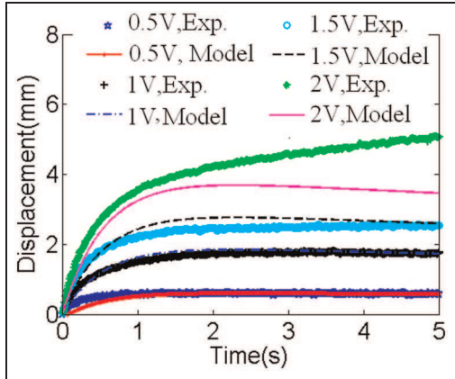
Figure 22. Tip displacement comparison between the time-variant model and the experimental data under DC ( L_{\text{eff}} = 30 \text{ mm} ). DC: direct current.
