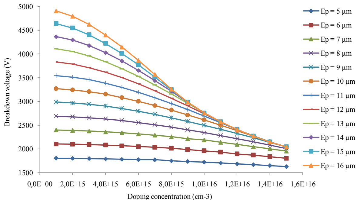
Fig. 2: Breakdown voltage for an ideal schottky diode (one dimensional simulation). Ep present the P- thickness layer of the diode.
