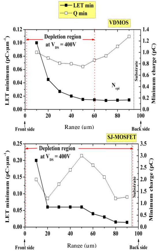
Fig. 6. Minimum LET and quantity of charges triggering a SEB depending on the penetration depth of the ion coming from the front side in normal incidence ( V_{DS}=400\text{ V} ) for standard (top) and SJ (bottom) MOSFETs
