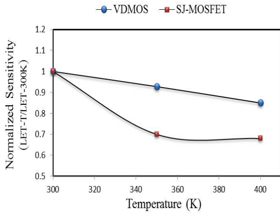
Fig. 11. Comparison of the sensitivity at different temperature value (minimum LET (T)/LET (T°)) with ion range=70μm
