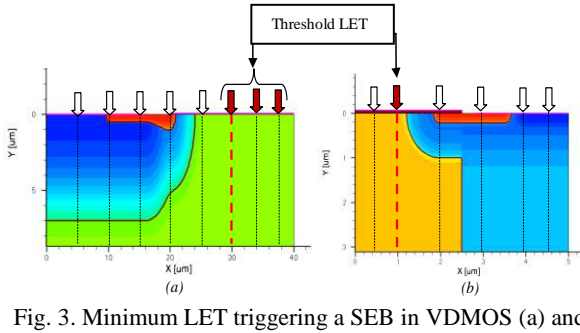
Fig. 3. Minimum LET triggering a SEB in VDMOS (a) and SJ-MOSFET (b) for various impact position ( x = \text{variable} , y = 0 , range = 10\mu\text{m} , V_{DS} = 400\text{ V} )
