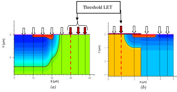
Fig. 3. Minimum LET triggering a SEB in VDMOS (a) and SJ-MOSFET (b) for various impact position ( x = \text{variable} , y = 0 , range = 10\mu\text{m} , V_{DS} = 400\text{ V} )
