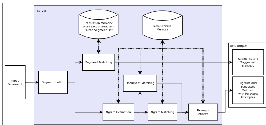
Fig. 2. TermWise Client-Server Architecture
