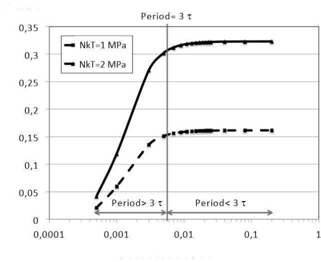
Fig. 7 Test #5: stabilized value of \hat{\theta} versus loading frequency.
