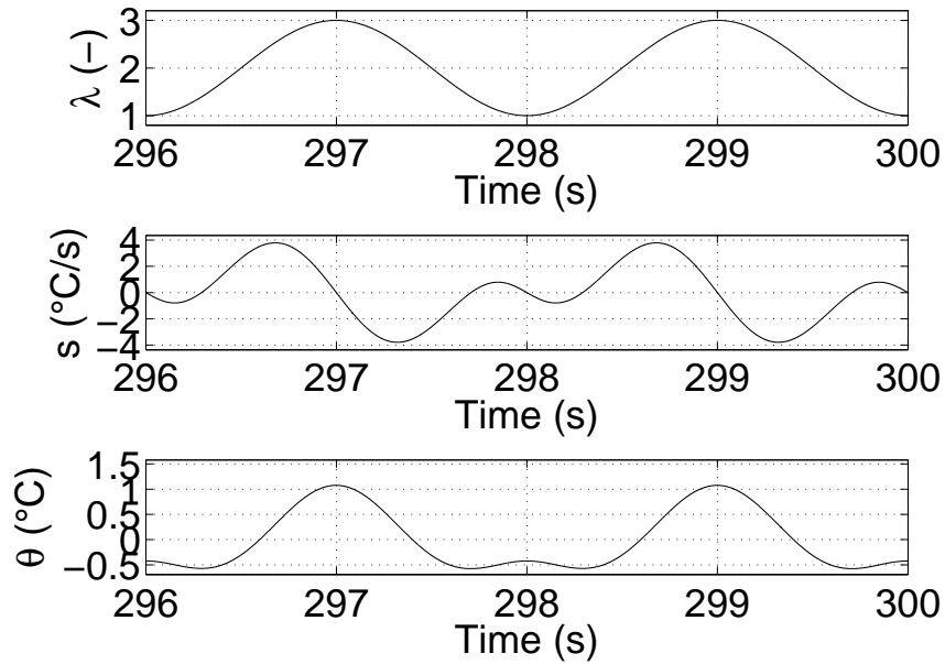
Fig. 11 Test similar to test #2 but accounting for isentropic coupling. Top: stretch ratio \lambda vs. time. Middle: heat source s vs. time. Bottom: temperature variation \theta vs. time.
