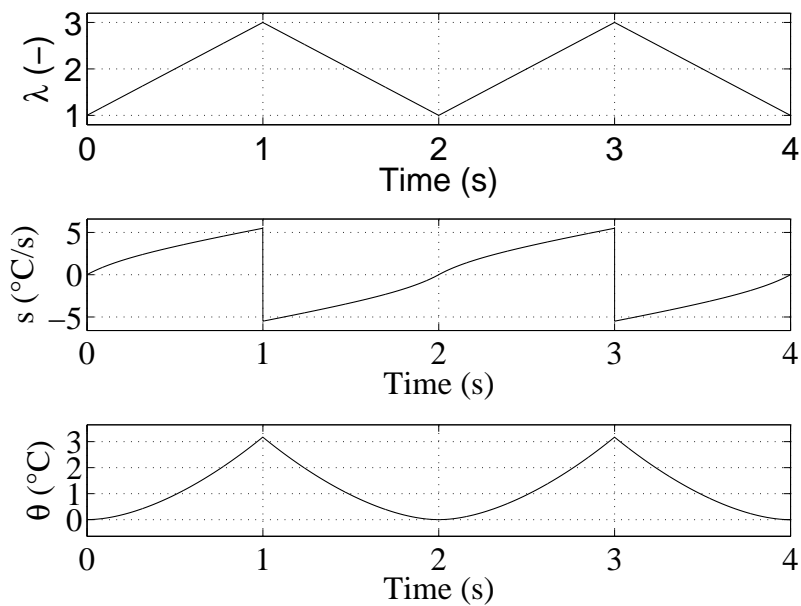
Fig. 1 Test #1 (adiabatic conditions, triangular signal, \lambda_{min} = 1 , \lambda_{max} = 3 , R_{\epsilon} = 0 , f = 0.5 \text{ Hz} ). Top: stretch ratio \lambda vs. time. Middle: heat source s vs. time. Bottom: temperature variation \theta vs. time.
