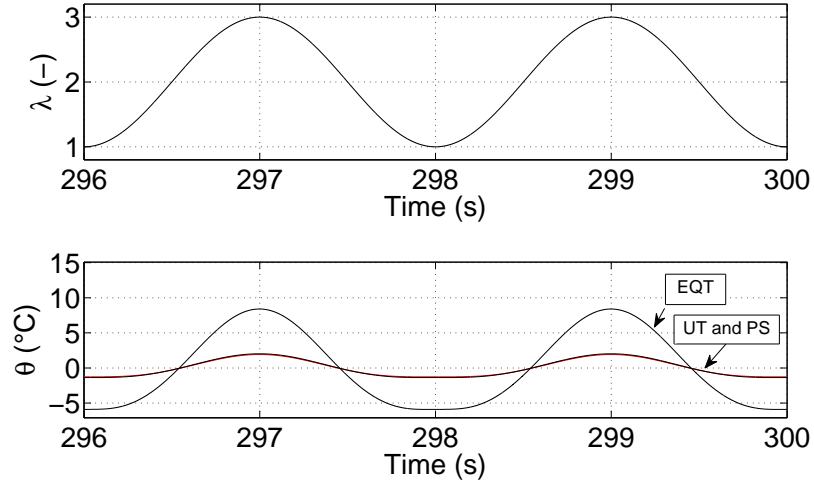
Fig. 10 Results obtained under uniaxial tension (UT), pure shear (PS) and equi-axial tension (EQT) for the last two cycles for non-adiabatic conditions. The other parameters are those used for test #4. Top: stretch ratio \lambda vs. time. Bottom: temperature variation \theta vs. time.
