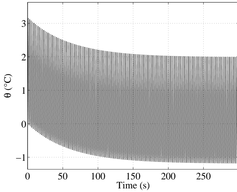
Fig. 3 Test #3 (non-adiabatic conditions, triangular signal, \lambda_{min} = 1 , \lambda_{max} = 3 , R_\epsilon = 0 , f = 0.5 Hz). Temperature variation \theta vs. time.
