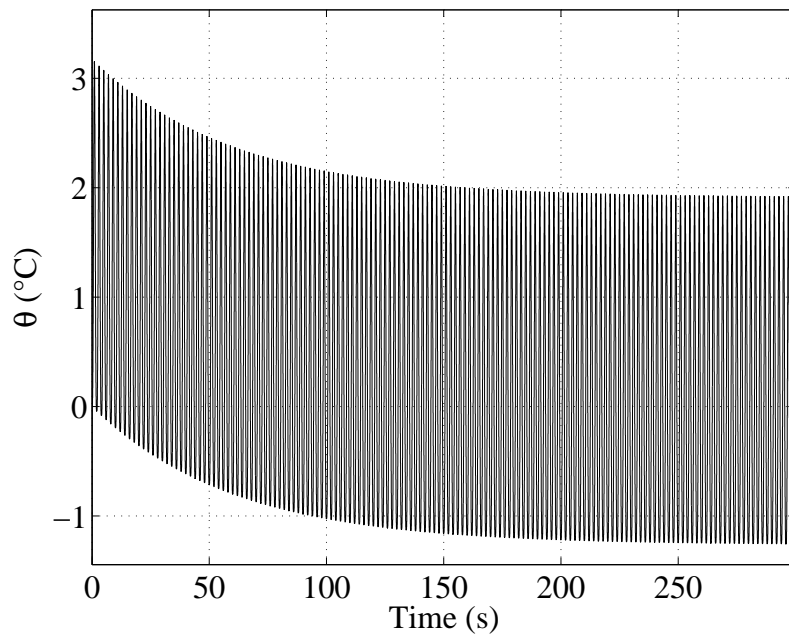
Fig. 5 Test #4 (non-adiabatic conditions, sinusoidal signal, \lambda_{min} = 1 , \lambda_{max} = 3 , R_\epsilon = 0 , f = 0.5 Hz). Temperature variation \theta vs. time.
