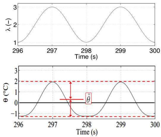
Fig. 6 Last two cycles of test #4.
