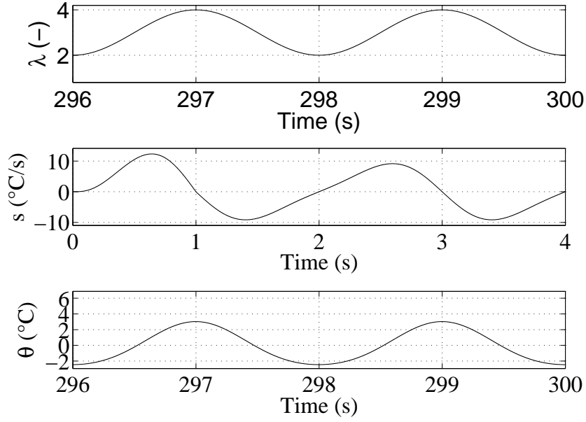
Fig. 9 Last two cycles of test #6.
