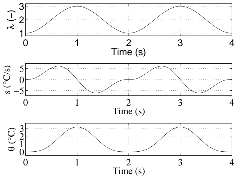
Fig. 2 Test #2 (adiabatic conditions, sinusoidal signal, \lambda_{min} = 1 , \lambda_{max} = 3 , R_{\epsilon} = 0 , f = 0.5 \text{ Hz} ). Top: stretch ratio \lambda vs. time. Middle: heat source s vs. time. Bottom: temperature variation \theta vs. time.
