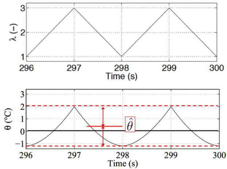
Fig. 3 Test #3 (non-adiabatic conditions, triangular signal, \lambda_{min} = 1 , \lambda_{max} = 3 , R_\epsilon = 0 , f = 0.5 Hz). Temperature variation \theta vs. time.
