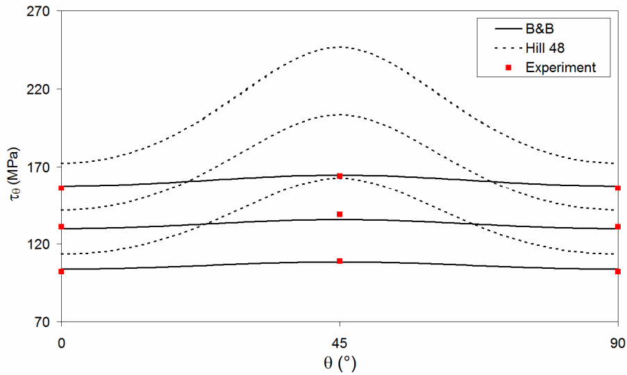
Fig. 5 Experimental and predicted shear stresses
