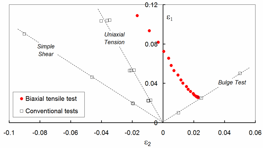
Fig. 17 Strain paths for the two identification methods
