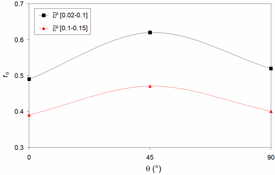
Fig. 2: Anisotropic coefficients calculated over two different equivalent plastic strain ranges
