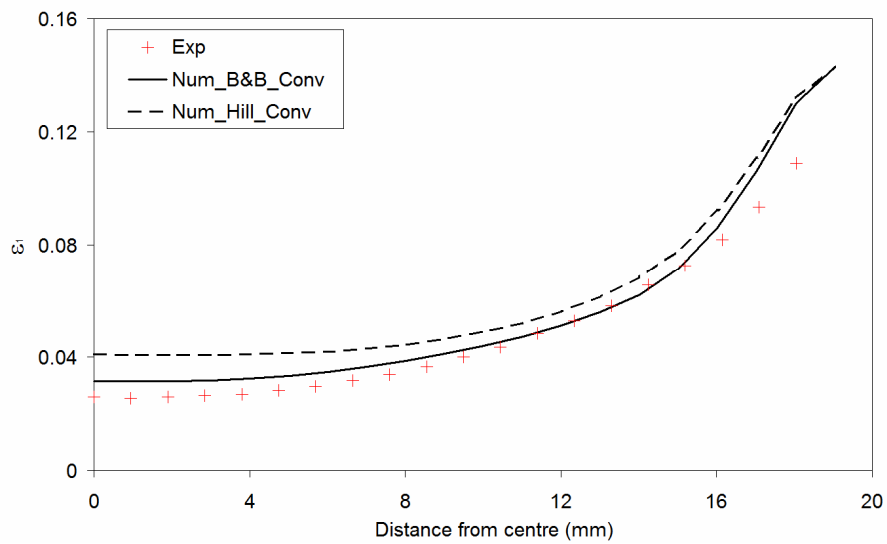
Fig. 15(a) Major strain
