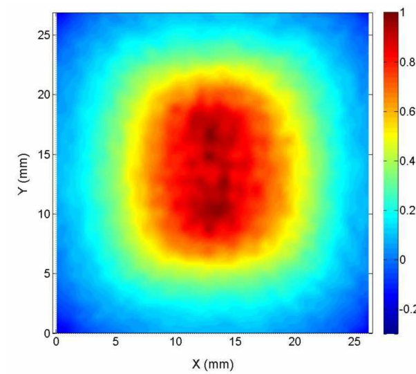
Fig. 9 Strain path ratio distribution \varepsilon_2/\varepsilon_1 in the analyzed central section
