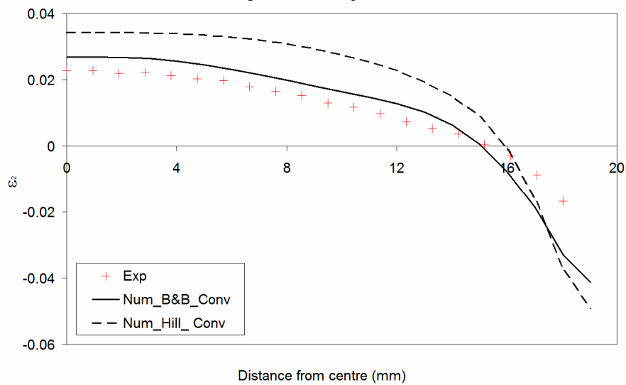
Fig. 15(b) Minor strain
