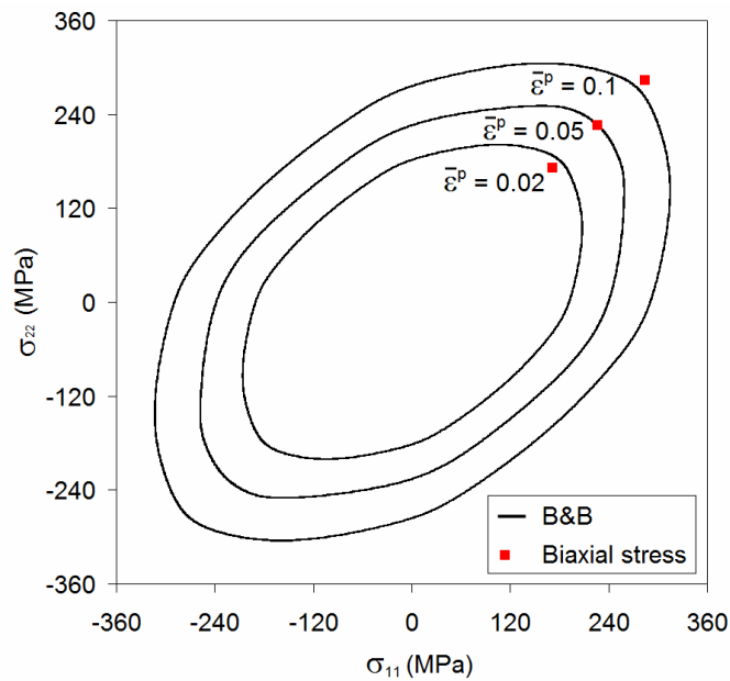
Fig. 6 Predicted yield surface contours
