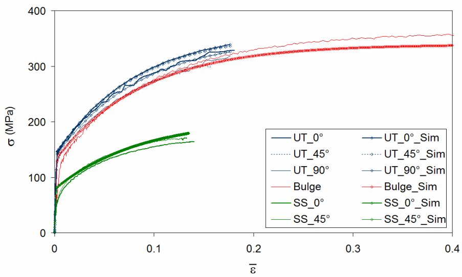
Fig. 18 Prediction of stress-strain curves for conventional tests using parameter set (Table 5) identified from the biaxial test
