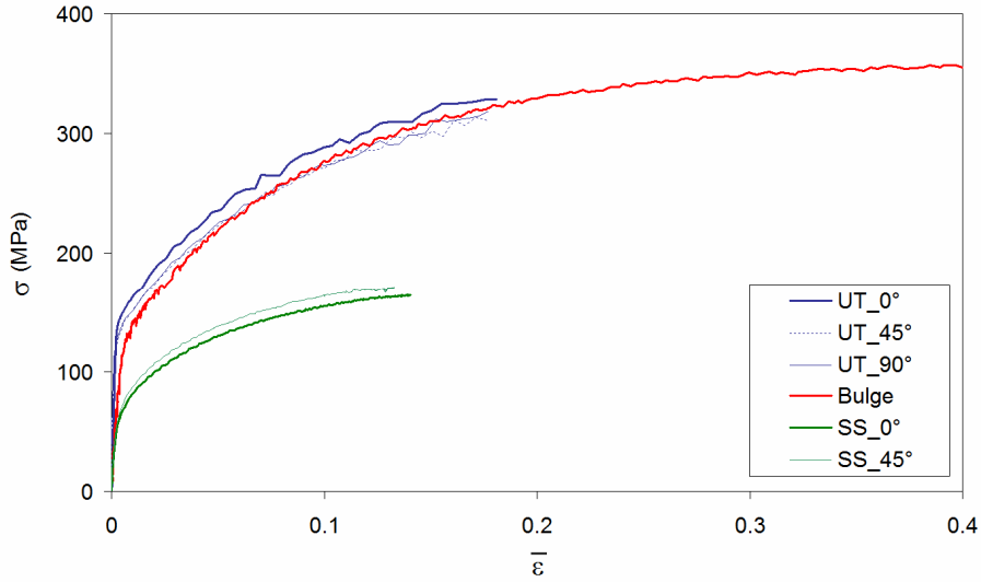
Fig. 1: Cauchy stress versus equivalent strain curves for conventional tests
