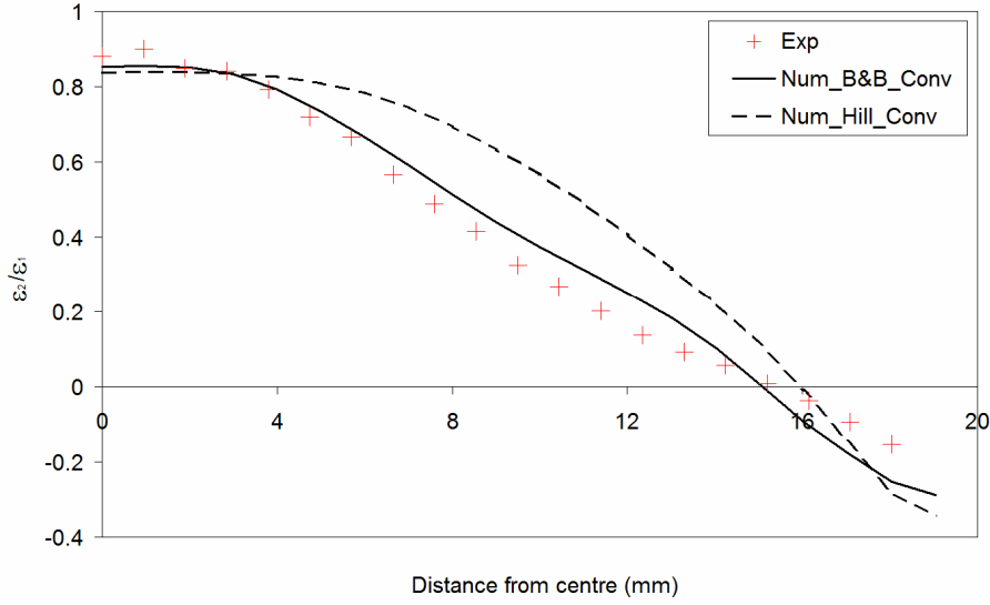
Fig. 15(c) Strain path ratio
