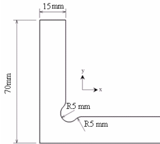
Fig. 7: Geometry of quarter cruciform specimen
