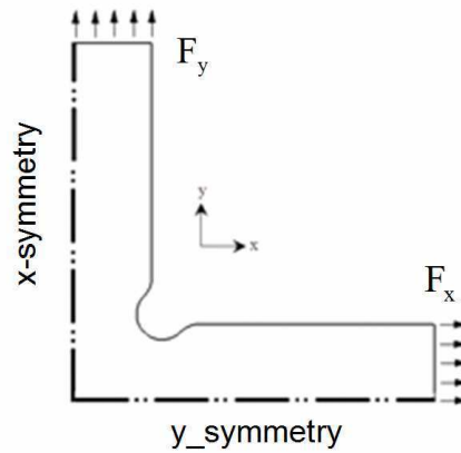
Fig. 13: FE boundary conditions
