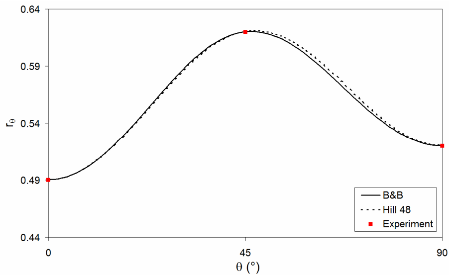
Fig. 3: Experimental and predicted anisotropic coefficients
