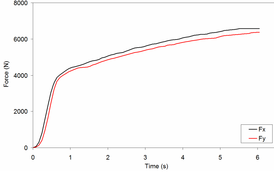
Fig. 12 Evolution of loads on the two arms
