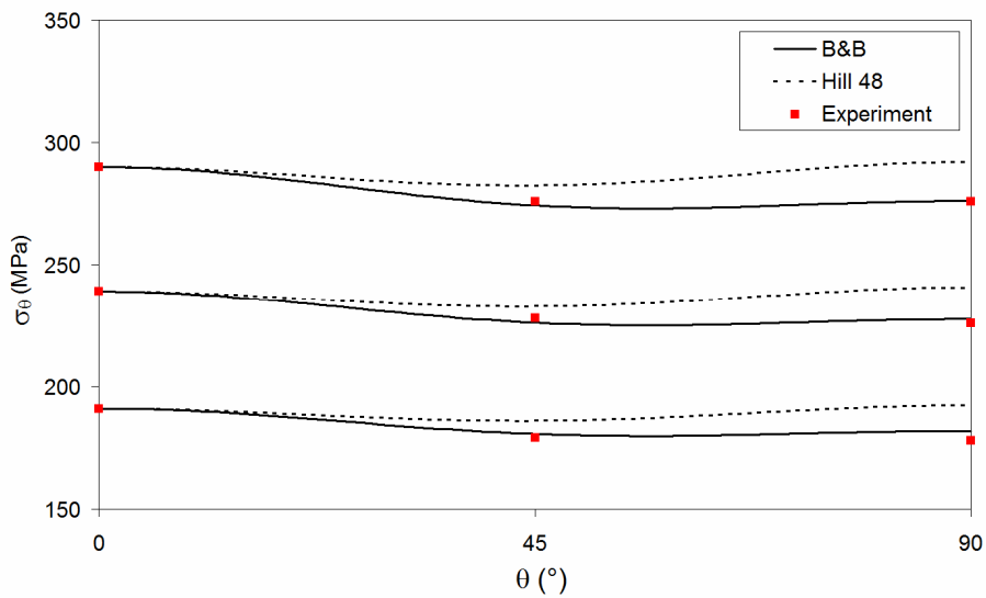
Fig. 4 Experimental and predicted uniaxial stresses
