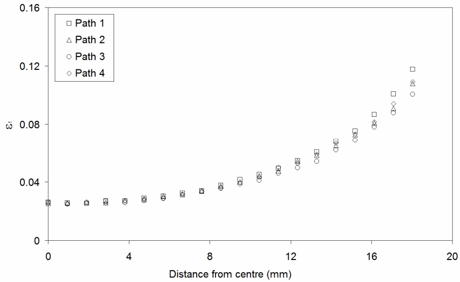
Fig. 10 Maximum principal strain along the four diagonal paths
