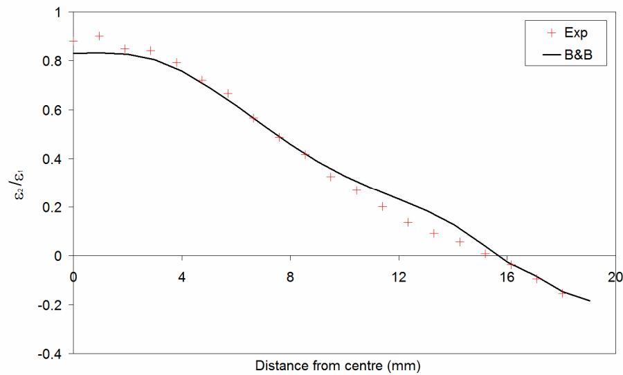
Fig. 16(b) Strain path ratio predicted by Bron and Besson yield function with parameters identified from the biaxial test
