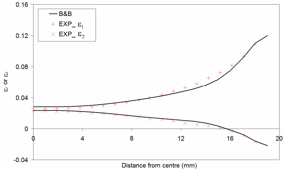
Fig. 16(a) Principal strains predicted by Bron and Besson yield function with parameters identified from the biaxial test
