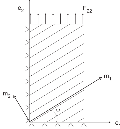
Fig. 3. Geometry of uniaxial tensile test in relation with anisotropy orientation \psi
