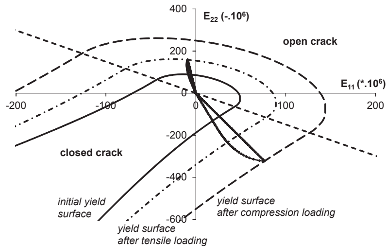
Fig. 7. Evolution of damage criteria f(F^{d^r}, d^r)=0 in (E_{11}, E_{22}) strain space for anisotropy orientation \psi=0 and for one crack orientation \phi^r=45 due to traction-compression loading represents by diamond symbols
