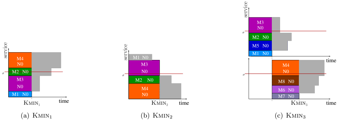
Figure 6: Lower bounds
