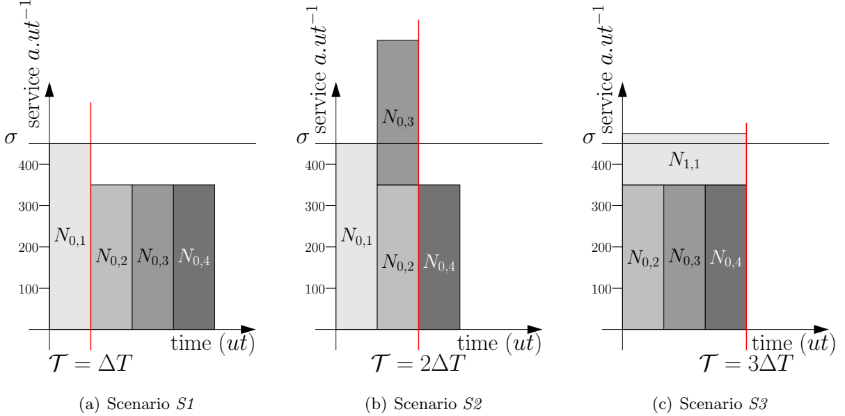
Figure 2: Motivating example
