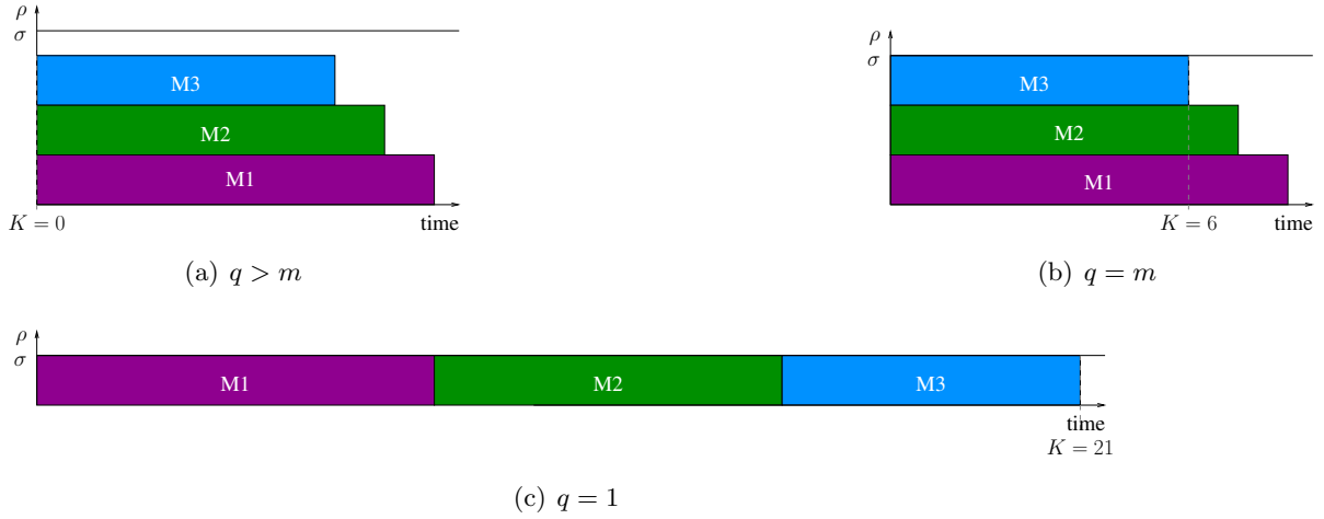
Figure 4: Straightforward cases
