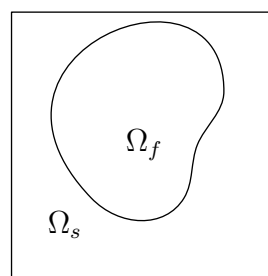
Figure 2: Schematic of fluid domain \Omega_f and penalised domain \Omega_s in computational domain \Omega = \Omega_f \cup \Omega_s .
