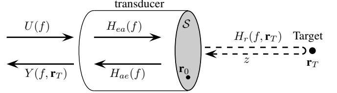
Fig. 2. Pulse-echo measurement for a target located at \mathbf{r}_T using a radiating surface \mathcal{S} . The received signal Y(f, \mathbf{r}_T) is modeled through a set of transfer functions: Y(f, \mathbf{r}_T) = U(f) H_{ea}(f) H_r(f, \mathbf{r}_T) H_{ae}(f) . z is the overall propagation distance.
