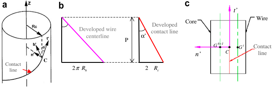
Fig. 4. (a) Local coordinate system R_C(C, \vec{t}', \vec{n}', \vec{b}') , (b) relation between the lay angle of a helical wire centerline and those of the contact line, and (c) linear contact core/wire.
