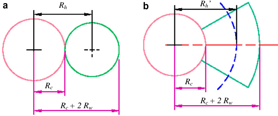
Fig. 5. The geometry considered by models: (a) present 1 + 6 model and (b) Leech's model (wedge geometry).
