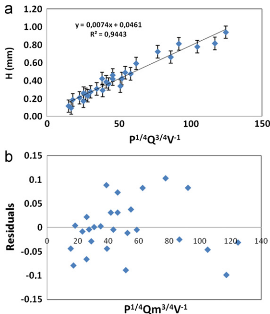
Fig. 8. (a) Laser track height H versus P^{1/4} Q_m^{3/4} / V^{-1} . (b) Residuals.
