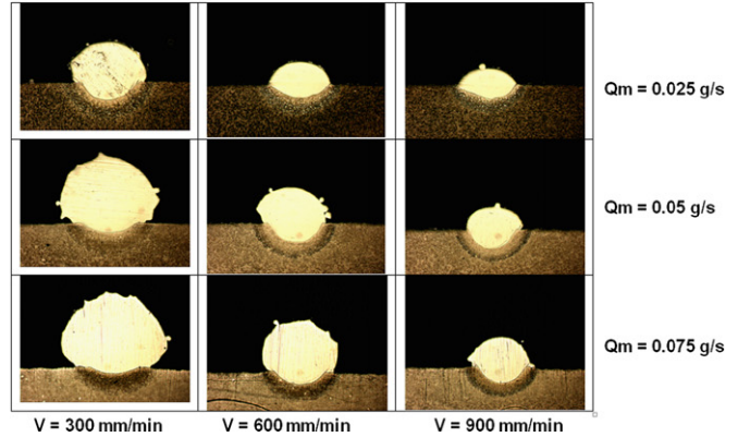
Fig. 7. All single tracks' cross-section. For each laser power the velocity ( V ) increases from the left to the right and the feed rate ( Q_m ) increases from the top to the bottom.
