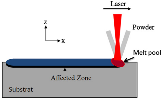
Fig. 1. Direct Laser Fabrication process.
