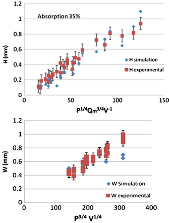
Fig. 17. Confrontation of the experimental height and width with the simulated results in the case of a Gaussian distribution.
