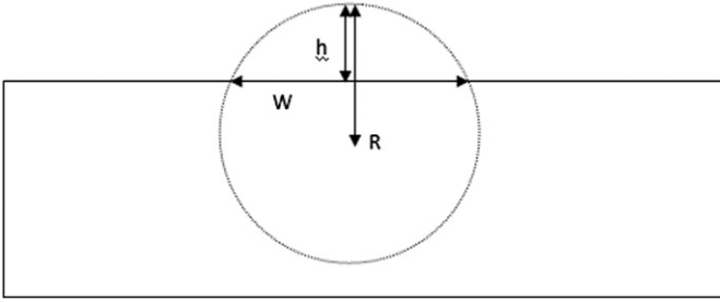
Fig. 18. Schematic view of the circular form model. The width W of the clad is the chord of the circle of radius R . h is the height of the deposit clad.
