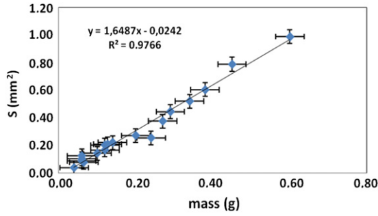
Fig. 11. Linear dependence between the surface of cross section and the clad mass at P=180 W and P=360 W.
