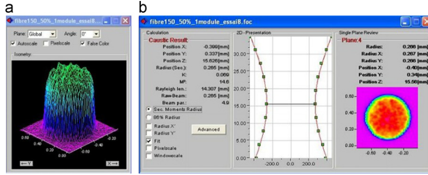
Fig. 3. Top hat laser beam analysis: (a) Spatial distribution of irradiance, (b) focalization plane determination and divergence of the laser beam.
