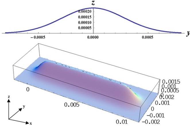
Fig. 14. Geometry of the deposited layer in case of a Gaussian powder distribution.
