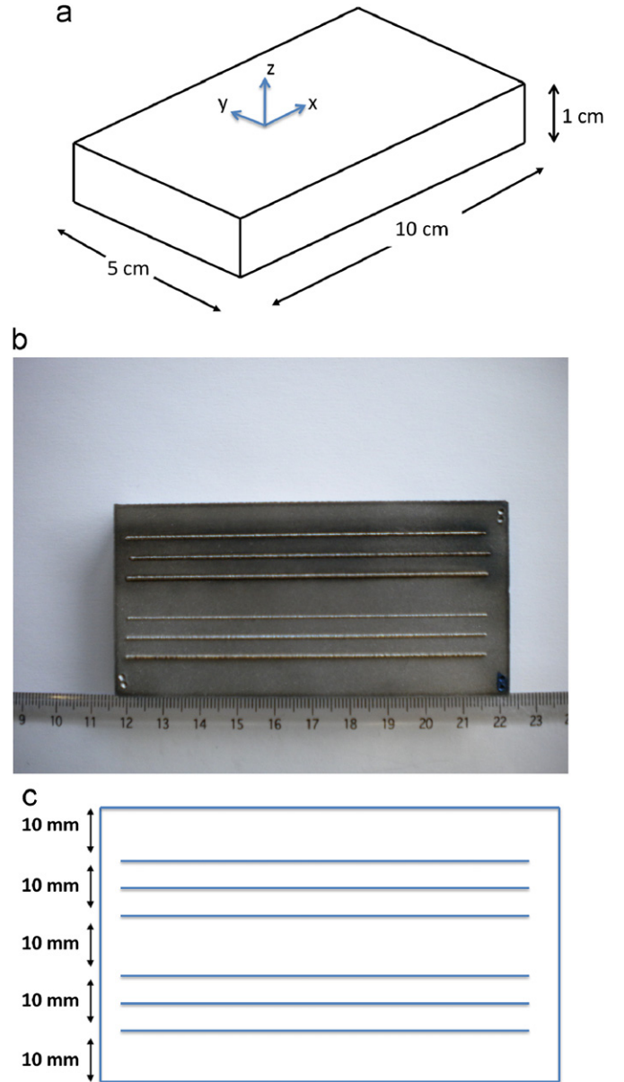
Fig. 5. (a) Substrate dimensions. (b) Image showing single tracks on a steel substrate. (c) Single track deposition on the substrate.
