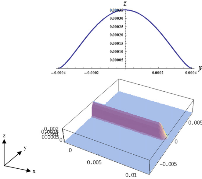
Fig. 15. Geometry of the deposited layer in case of a polynomial distribution.
