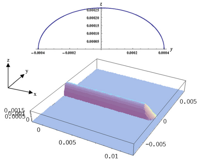
Fig. 13. Geometry of the deposited layer in case of a uniform powder distribution.
