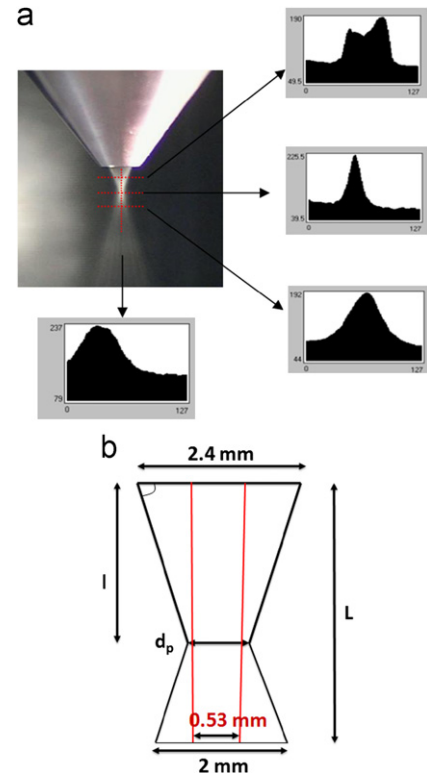
Fig. 2. (a) Powder stream pictures analysis. (b) Powder cone shape from the nozzle issue to the laser focused plan.
