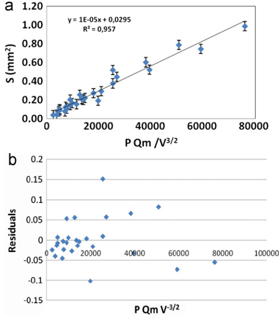
Fig. 10. (a) Clad area versus P Q_m / V^{3/2} . (b) Residuals.
