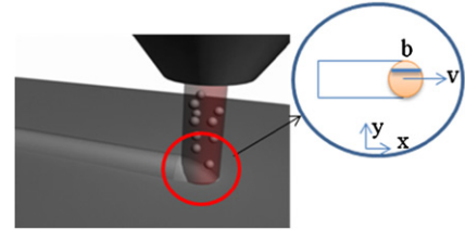
Fig. 12. Powder deposition on the substrate surface.
