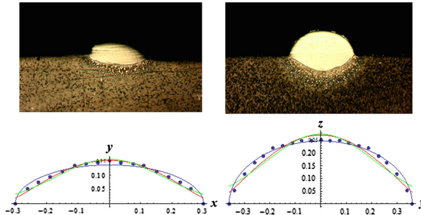
Fig. 16. Fitting with the three different functions to describe our experimental results.
