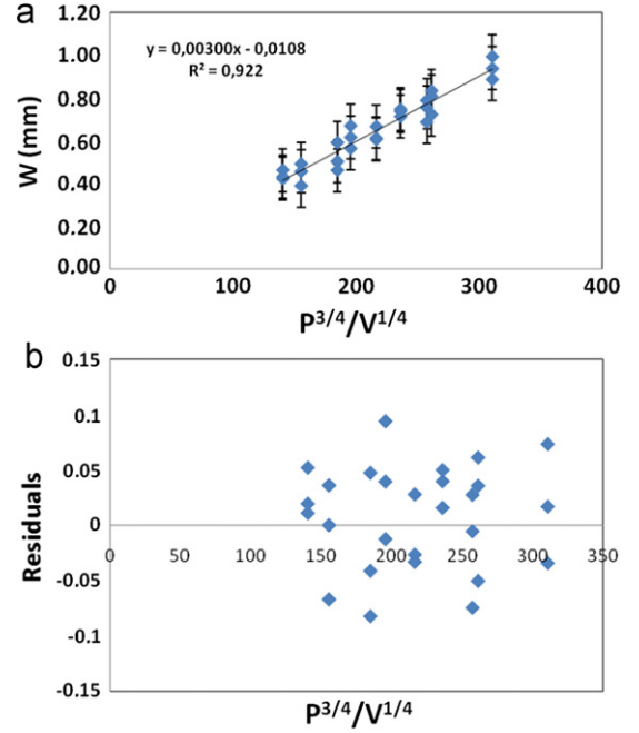
Fig. 9. (a) Clad width versus P^{3/4} V^{1/4} . (b) Residuals.
