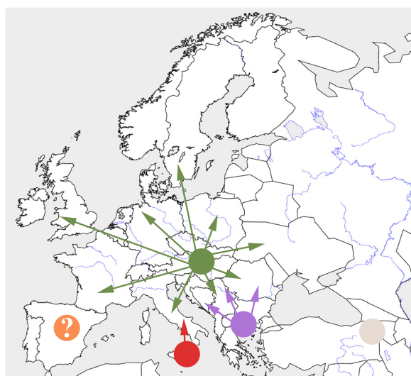
Figure 5 Scenario of the recent history of B. lapidarius .
