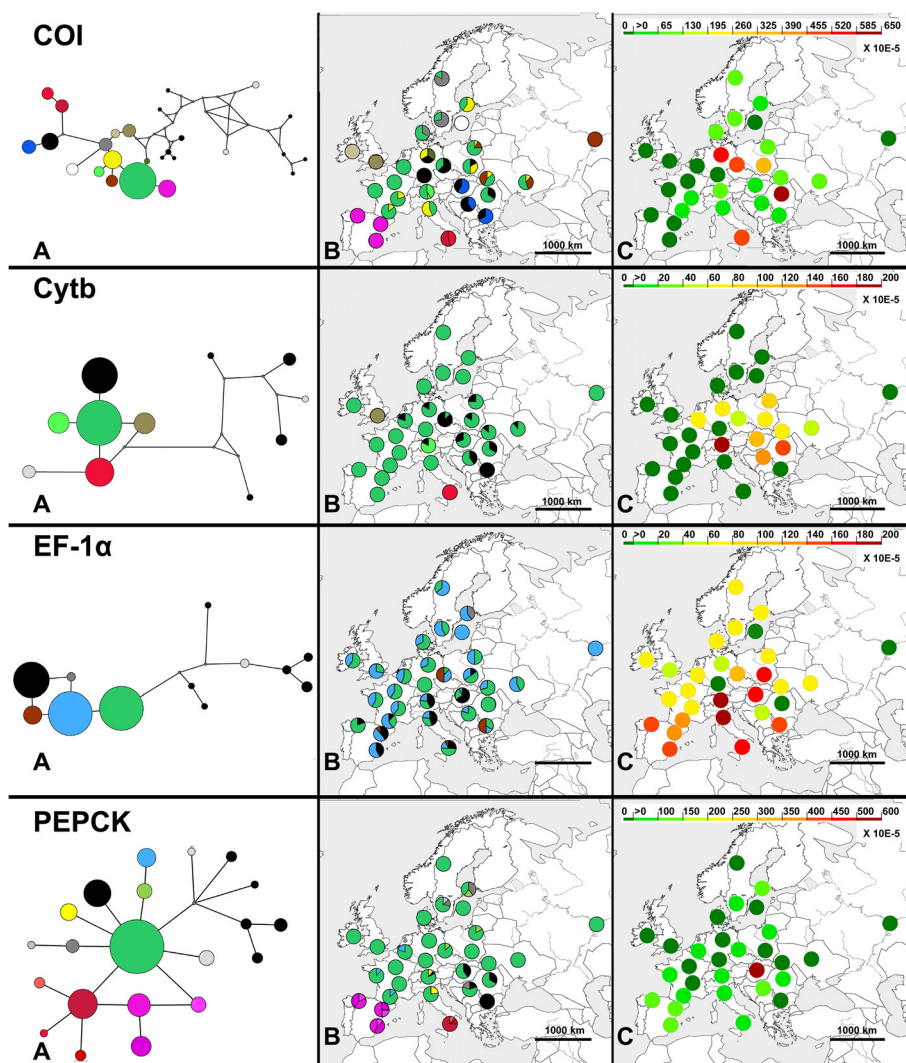
Figure 2 Geographic distribution of genetic diversities in B. lapidarius . In the left column median-joining network of haplotypes based on COI , Cytb , EF1α , and PEPCK are coloured by haplotypes. In the centre column maps of haplotype frequency for each geographic groups based on COI , Cytb , EF1α , and PEPCK have the colours of pie charts as for haplotype colour (left column). In the right column maps of nucleotide diversity for each geographic group based on COI , Cytb , EF1α , and PEPCK , Colours of pie charts refer to coloured intensity scale.
