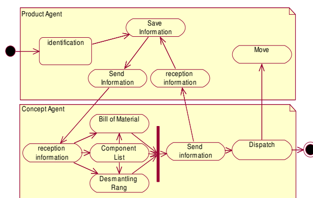
Fig. 5 UML Activity Diagram: design agent
