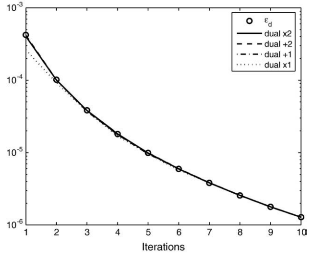
Fig. 3. Error evolution associated with Problem 1 .
