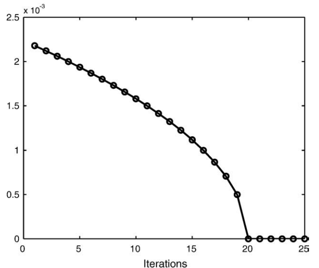
Fig. 2. Evolution of the residual L^2 -norm.
