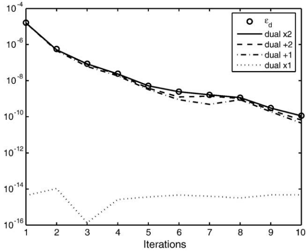
Fig. 5. Error evolution associated with Problem 3.
