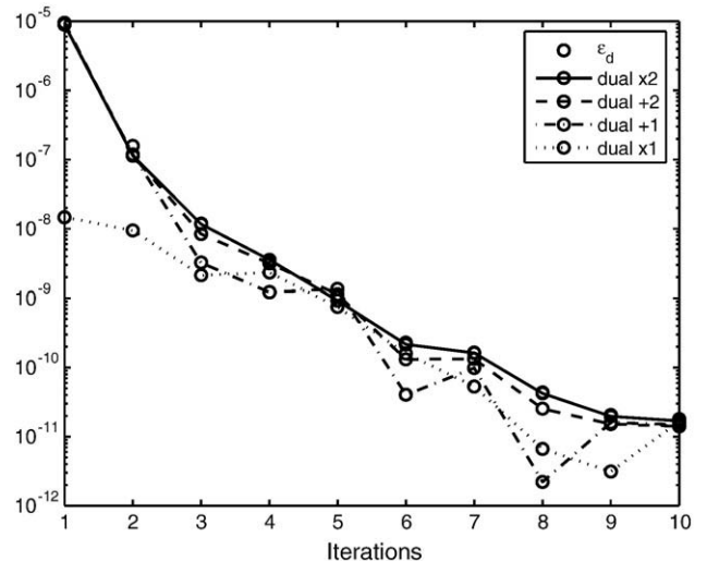
Fig. 4. Error evolution associated with Problem 2 .
