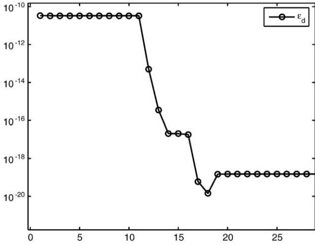
Fig. 8. Evolution of the estimated error for the 10D problem.
