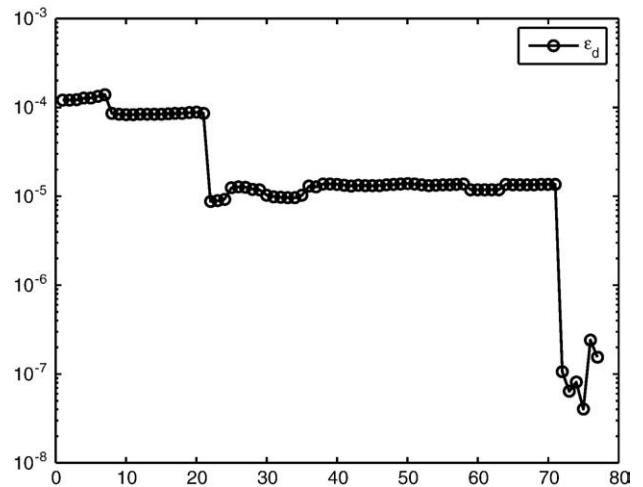
Fig. 7. Evolution of the estimated error.
