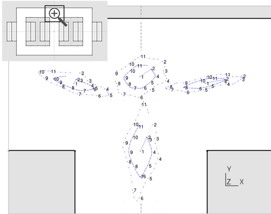
Fig. 6. Magnetic and induction field in the central T -joint of a three-phase transformer over about one period. The dotted line is the \mathbf{h} -field and the solid line is the \mathbf{b} -field obtained with three internal variables \mathbf{J}^k (cf. Table 1(a)).
