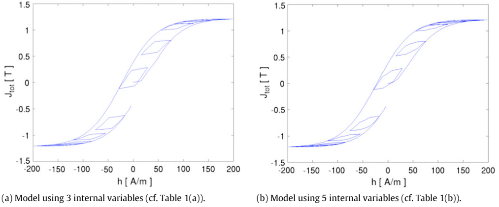
Fig. 4. Main and minor hysteresis loops of M250-50A steel modeled with 3 or 5 internal variables, when a 10-th harmonic is superimposed to the main frequency.
