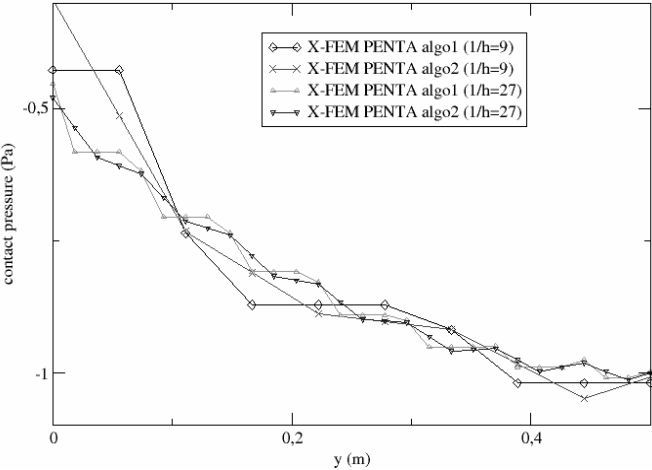
Figure 8. Comparison of the contact pressure for both algorithms on half-length of the structure
