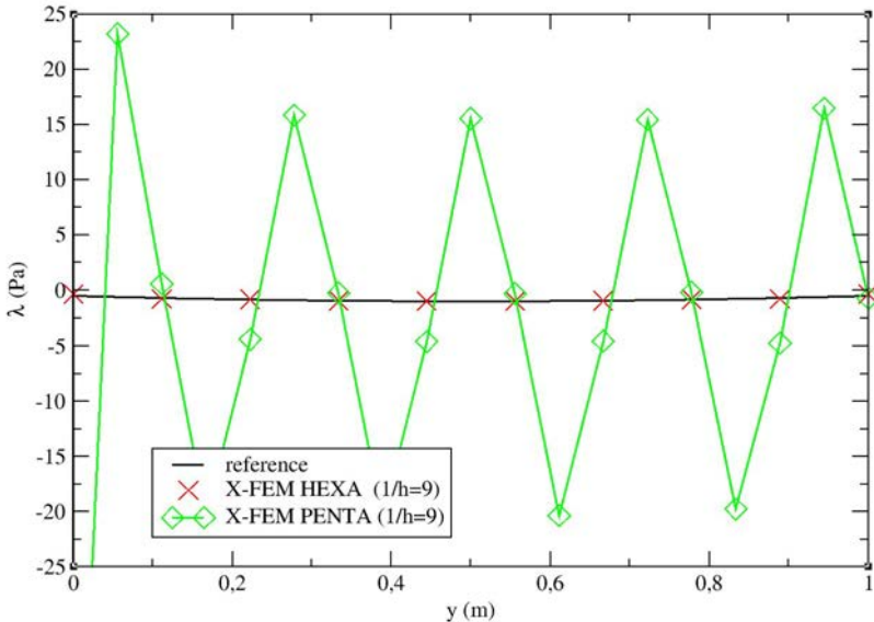
Figure 5. Contact pressure oscillations
