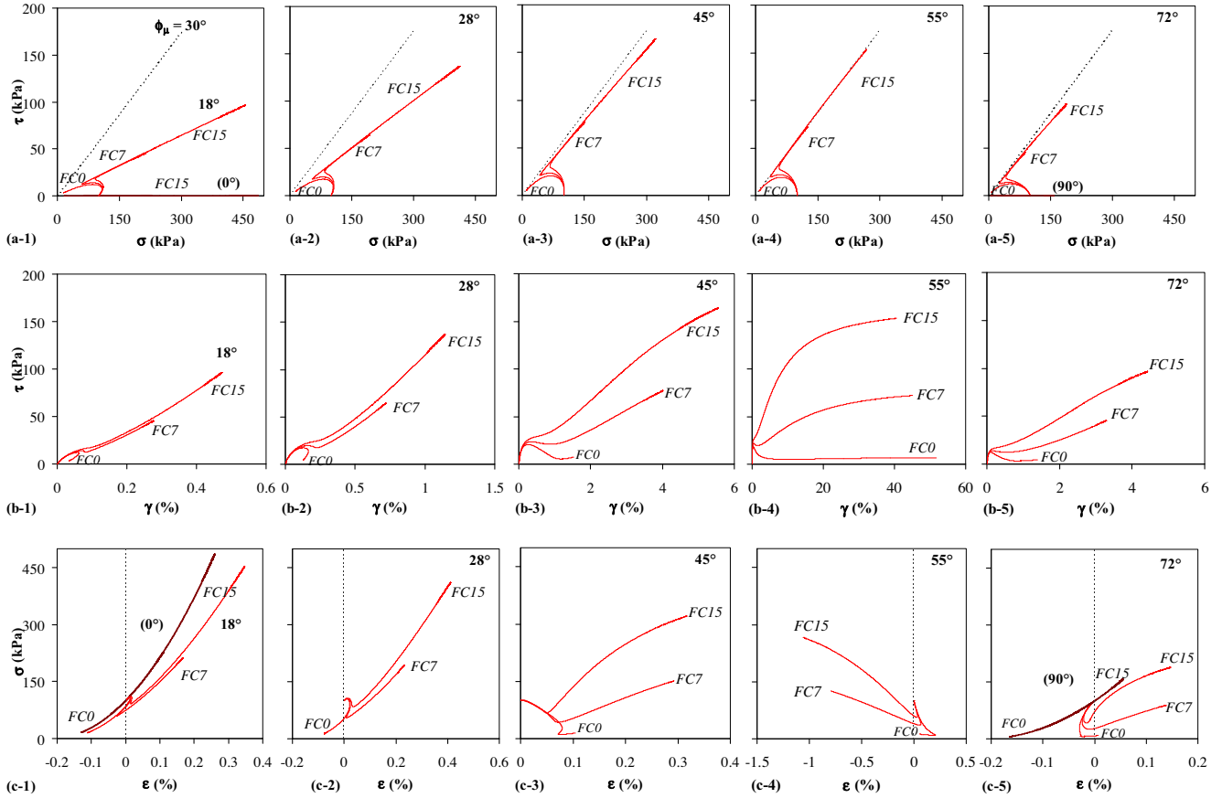
Fig. 12. Local stress-strain behavior of silty sand with an inter-granular void ratio of 0.8.
