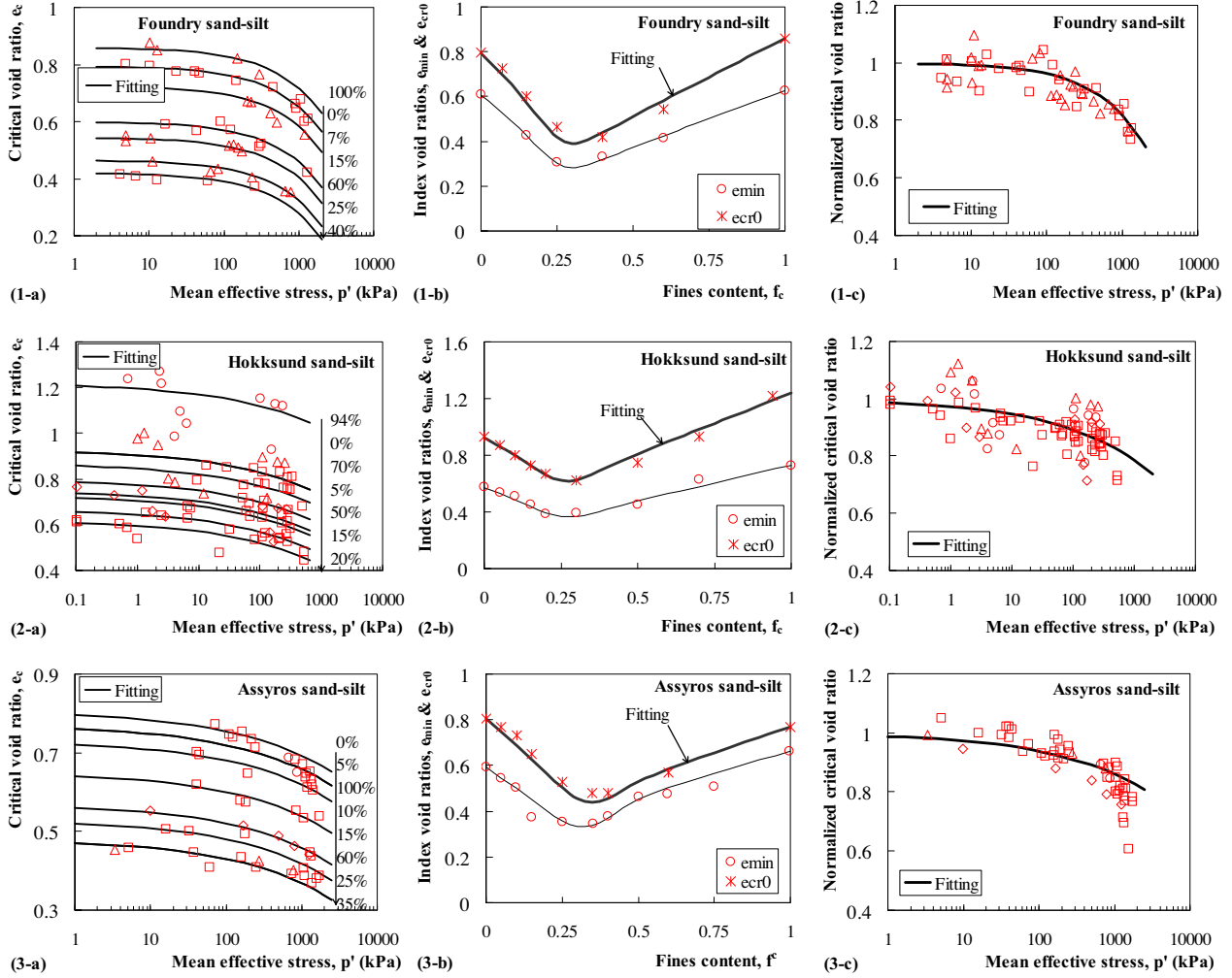
Fig. 4. Critical state lines of three sand-silt mixtures: (a) Critical state lines in e - \log p' plan, (b) Initial critical void ratio versus fines content, and (c) Normalized critical state lines.
