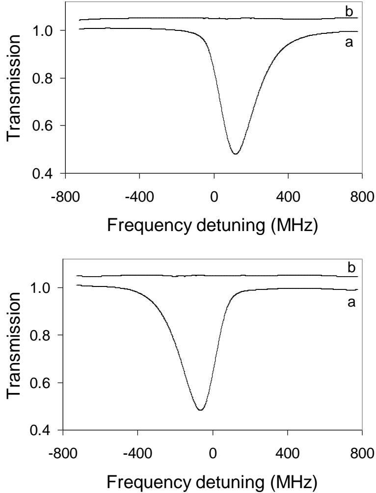
FIG. 2. Transmission of the saQ(6,3) rovibrational line of the \nu_2 vibrational mode of ^{14}\text{NH}_3 recorded for increasing (upper panel) and decreasing (lower panel) frequencies (see text for details). (a): recorded line; (b): unmagnified residuals from a Voigt profile fit taking the detection system properties into account ( \Delta\nu_{col} = 13.60(8) and 12.56(7) MHz, respectively, achieved signal-to-noise ratios \approx 480 and 550 , respectively). Frequency scale (in MHz) is shifted by 28.953\,600 THz; temperature \approx 273.15 K; pressure \approx 1 Torr; cell length = 4.5 cm; frequency step \Delta\nu = 1.5 MHz; step duration \Delta t = 68.8 ms; indicated lock-in time constant \tau_D = 3 s.
