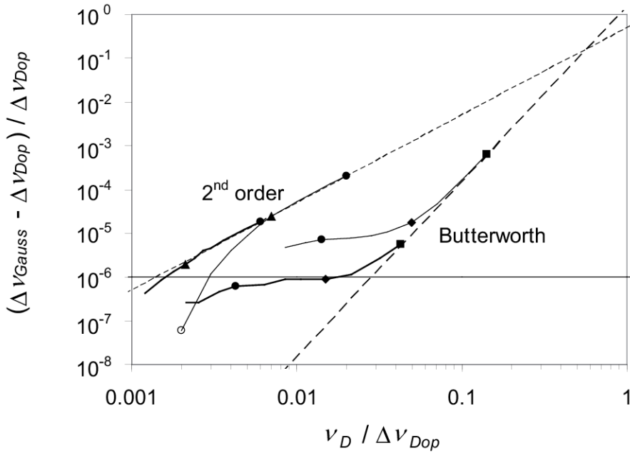
FIG. 8. Influence of frequency sweeping conditions on the Doppler broadening determination (2 nd order filters with Q = 1/2 and \sqrt{1/2} (Butterworth case)). Relative broadening deviations are plotted versus frequency constant v_D / \Delta v_{Dop} . Frequency step \Delta v / \Delta v_{Dop} = 0.003 (thick line) and 0.01 (thin line) are drawn. For convenience, some \tau_D / \Delta t ratios are specified by symbols: (○) 0.1; (▲) 0.35; (●) 1.0; (◆) 3.5; (■) 10. Thin and thick dotted lines refer to continuous frequency sweeping models ( Q = 1/2 and \sqrt{1/2} , respectively). The 1 ppm target is depicted by the horizontal solid line.
