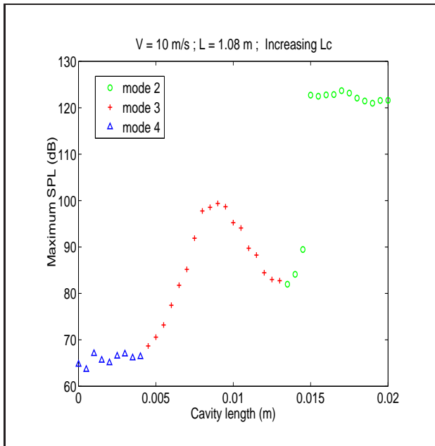
Figure 2. Maximum SPL measured in the pipe 1cm from the air inlet as a function of the cavity length
