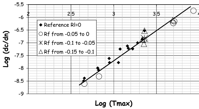
Figure 2. Crack growth curve measured with DSS (Double Simple Shear) sample. The displacement is enforced and the reference is obtained with relaxing conditions R_1 = L_{min}/L_{max} = 0 . The tensile compressive loading results are superimposed to the reference curve.
