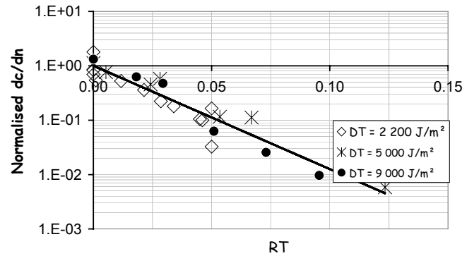
Figure 4. Identification of the g(R_T) .
