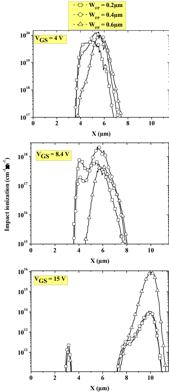
Figure 9: Impact ionization along the STI/SOI interface for different values of the W_{FP} at three different V_{gs} in the striped STI LDMOS transistor
