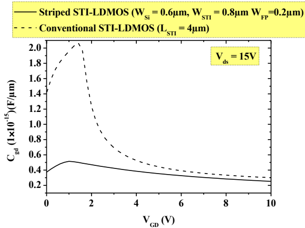
Figure 6: C_{gd} as a function of V_{gd} for both LDMOS structures
