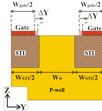
Figure 10: Cross section detail (through the P-well/STI Y axis) of a Striped STI-LDMOS cell showing the possible mask misalignment between the poly gate and the STI indicated by the parameter \Delta Y .
