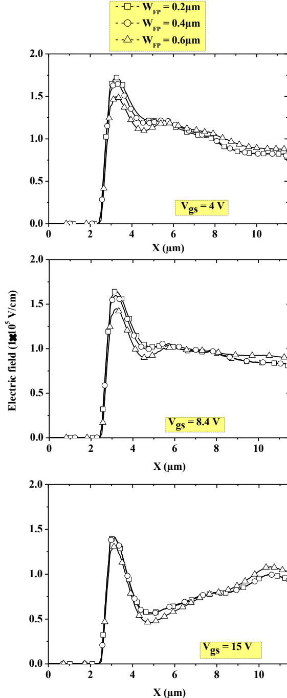
Figure 8: Electric field distribution along the STI/SOI interface for different values of the W_{FP} at three different V_{gs} in the Striped STI LDMOS transistor
