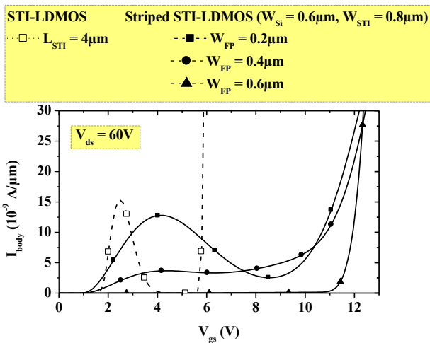
Figure 7: I_{body} characteristics vs V_{gs} for both LDMOS structures at high applied V_{ds} of 60V
