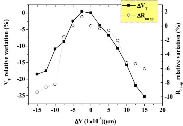
Figure 11: Relative variation of the R_{\text{on-sp}} and V_t as a function of the \Delta Y parameter.
