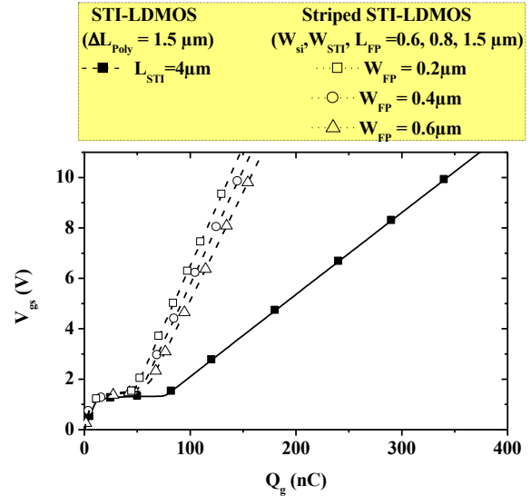
Figure 5: Gate voltage versus gate charge and R_{on} \times Q_g FOM
