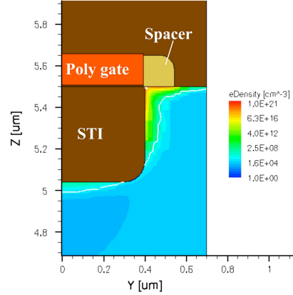
Figure 2: Electron distribution in the channel region of the striped STI-LDMOS
