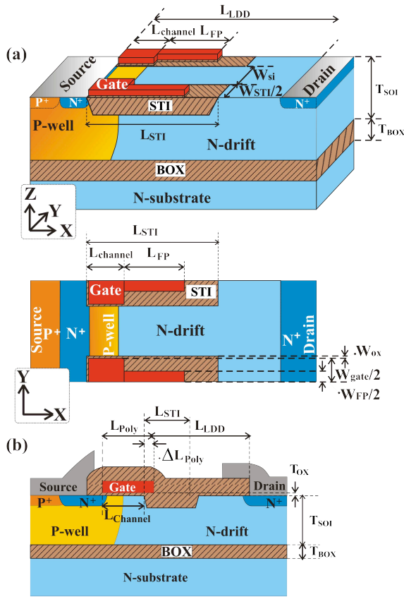
Figure 1: Schematic cross section of the (a) proposed striped STI-LDMOS and (b) conventional STI-LDMOS structures
