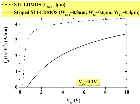
Figure 4: Drain current as a function of V_{gs} for both analyzed STI-LDMOS structures.
