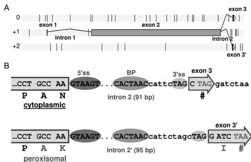
Figure 2. Gene model for YIMDH2 . (A) Schematic representation of alternative transcripts from the multi-intronic MDH gene YIMDH2 . Exons are represented by grey rectangles and introns are symbolized by thin black articulated lines. Vertical bars on each of the three phases (0, +1 and +2) represent in-frame stop codons. (B) Sequence representation of the 3' regions centred on the second intron. Coloured circles indicate the 5'-splice site, the BP and the two 3'-splice sites used to generate the two mRNA variants. Exon parts are represented by grey rectangles and the two putative C-terminal protein sequences are indicated.
