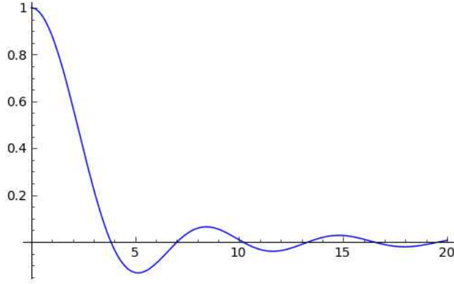
FIGURE 1. \Omega_4(t)
