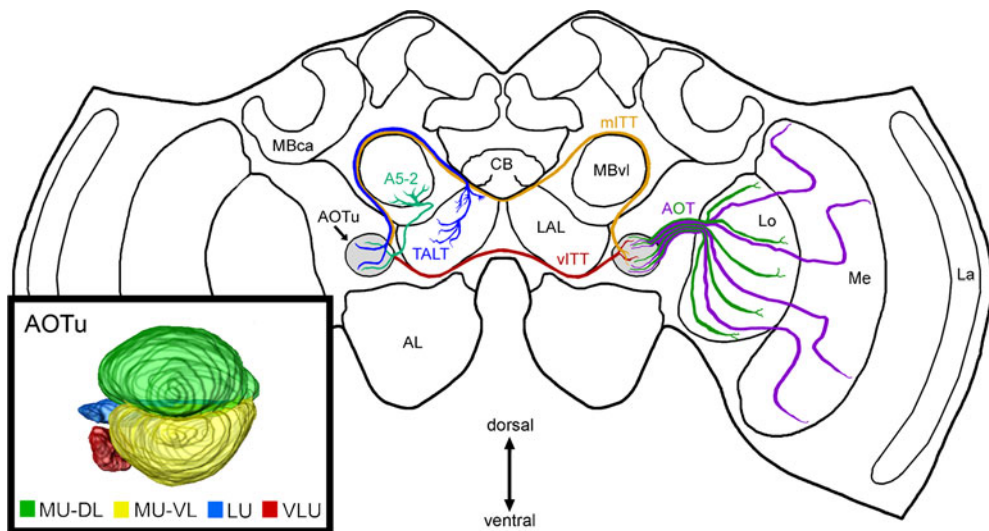
Figure 6. Three-dimensional structure and neural connectivity of the anterior optic tubercle (AOTu). Three-dimensional reconstruction showing the different AOTu compartments (left inset): major unit dorsal lobe (MU-DL; green), major unit ventral lobe (MU-VL; yellow), ventrolateral unit (VLU; red), and lateral unit (LU; blue). The schematic diagram summarizes neural pathways connecting the AOTu with other brain neuropils. La lamina, Me medulla, Lo lobula, AL antennal lobe, MBvl mushroom body vertical lobe, MBca mushroom body calyx, CB central body, LAL lateral accessory lobe, AOT anterior optic tract, vITT ventral inter-tubercle tract, mITT medial inter-tubercle tract, TALT tubercle-accessory lobe tract; A5-2 neuron previously described by Rybak and Menzel (1993).
