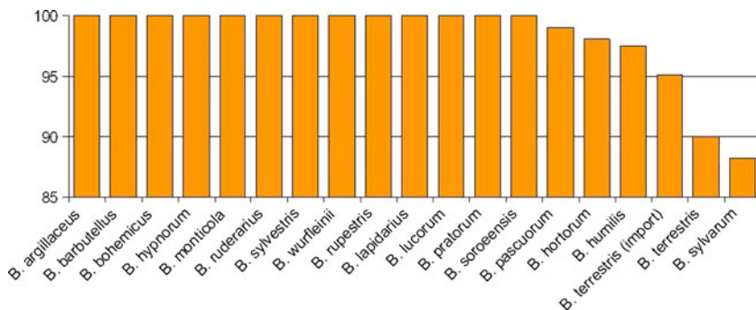
Figure 3. Percentage (%) of correctly assigned specimen based on discriminate analysis.
