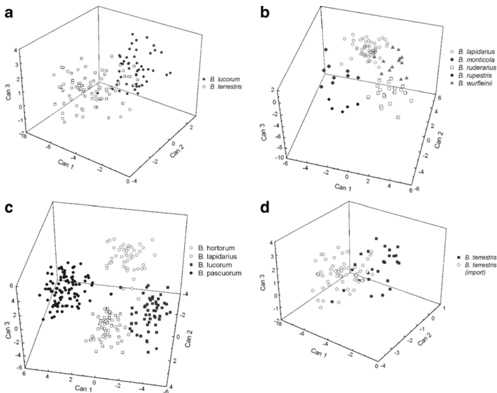
Figure 4. Differences in wing venation pattern based on discriminate analysis between different bumblebees species.
