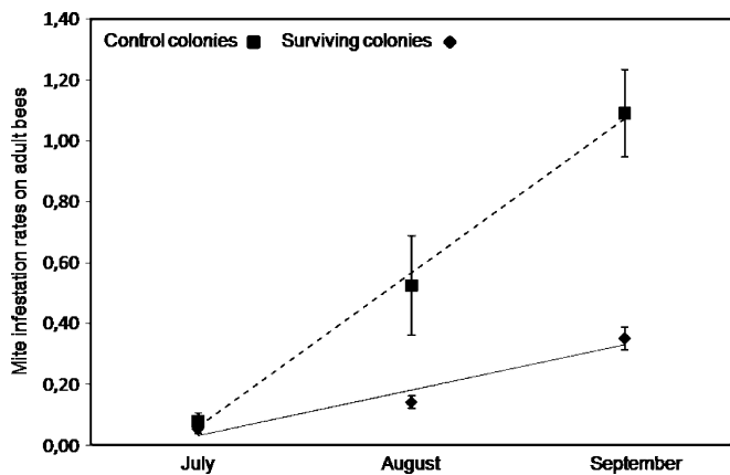
Figure 2. Regression lines on the mean mite infestation rates (number of mites per 200 adult bees) with standard error bars, in 2009, of surviving colonies ( solid line ; y=0.15x-0.12 ) through July ( n=13 ), August ( n=11 ) and September ( n=13 ), and for control colonies ( dotted line ; y=0.51x-0.45 ) through July ( n=11 ), August ( n=11 ) and September ( n=8 ) on Gotland.
