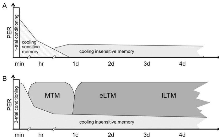
Figure 1. Appetitive olfactory memory in honeybees Apis mellifera . a A single olfactory conditioning trial induces a memory that is initially at a high level, decays within 1 day, and remains at a low level for several days. Memory performance is evaluated by PER. Cooling of the honeybees immediately after single-trial conditioning erases an early memory phase, defined and indicated as cooling-sensitive memory, while memory from about 1 day is not affected by cooling (cooling insensitive memory). The memory induced by a single-trial conditioning is insensitive to translation and transcription inhibitors. b Three conditioning trials applied within a few minutes induce a stable and long-lasting memory that consists of several mechanistically distinguishable phases. No cooling sensitive memory phase is detectable after 3-trial conditioning. An early cooling insensitive memory phase (not so far mechanistically characterised) is followed by a mid-term memory (MTM) from about 1 h to 1 day, and a subsequent long-term memory (LTM). The LTM can be divided into two phases, an early LTM (eLTM) and a late LTM (ILTM). eLTM requires only translation processes, ILTM requires both translation and transcription processes. Erasing MTM, eLTM, or ILTM by the appropriate treatments reduces memory performance to the level of the cooling-insensitive memory.
