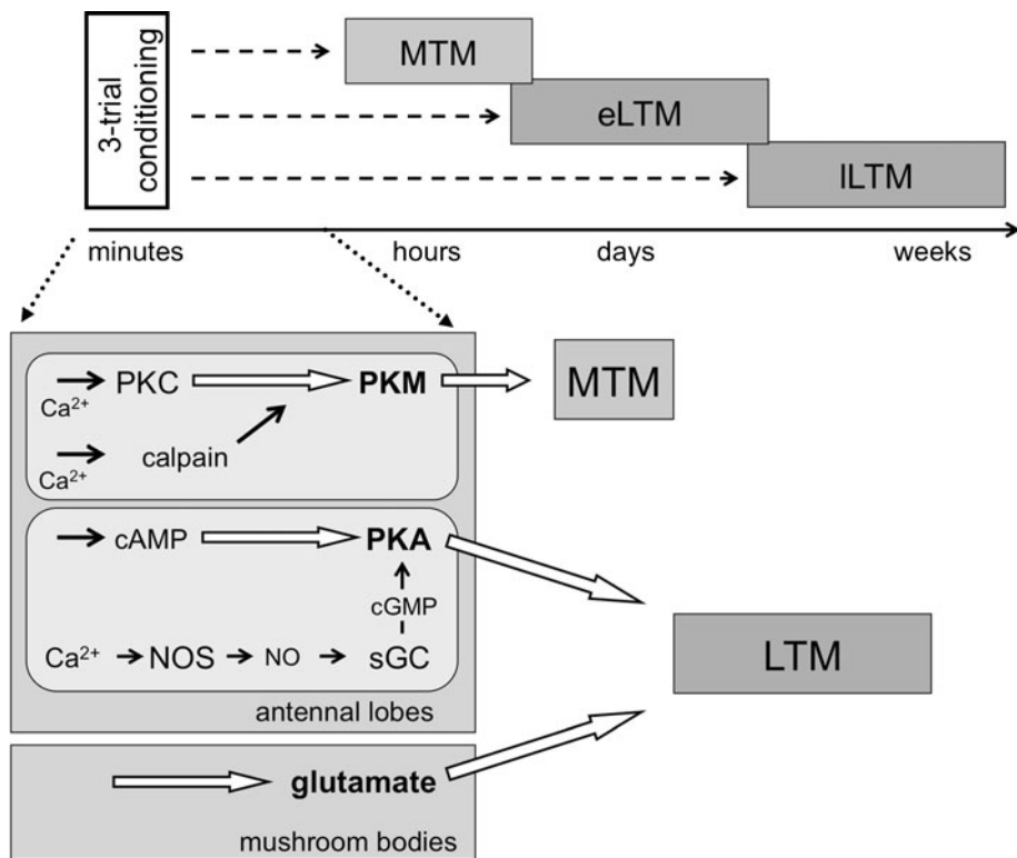
Figure 2. Parallel molecular processes contribute to the formation of different memory phases: MTM and LTM . In the antennal lobes, at least two independent processes contribute to the formation of two distinguishable memory phases. MTM Three-trial conditioning activates both the Ca 2+ -dependent protease calpain and the Ca 2+ /phospholipid-dependent protein kinase C ( PKC ). Activated calpain cleaves PKC , which results in the production of constitutively active protein kinase M ( PKM ). PKM , which remains active for hours, is required for mid-term memory ( MTM ). Blocking calpain leads to the specific loss of the MTM phase. LTM In an independent process, three-trial conditioning induces a prolonged activation of the protein kinase A ( PKA ) that is essential for the induction of long-term memory ( LTM ). Conditioning activates the formation of nitric oxide ( NO ), which in turn activates the soluble guanylyl cyclase ( sGC ) resulting in cGMP production. The synergistic action of cAMP and cGMP causes a prolonged PKA activation in the range of minutes, which is required for LTM formation. Blocking NOS , sGC , or PKA activation causes a specific loss of the LTM phase. In addition, glutamate-mediated processes located in the MBs contribute to LTM formation.
