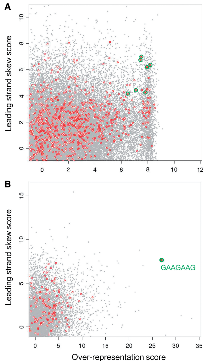
Figure 3. Prediction of the L. lactis KOPS motif. (A) Distribution of octamers with one degenerated position in the L. lactis chromosome. All octamers that have a positive over-representation and skew score and a minimal frequency of 1 every 70 kb on the whole chromosome are represented in grey. Among these, motifs that have a specific distribution in the dif region are shown in red. They represent the 100th most skewed motifs among those with a leading strand skew in the dif region higher than 90%, a minimal frequency of 1 occurrence every 40 kb in this region and a minimal frequency of 1 occurrence every 70 kb in the whole genome. The strength of the red represents the over-representation score in the dif region (the stronger the red, the more over-represented the motif). Four motifs stand out as potential KOPS candidates (highlighted in green) with three additional ones that are slightly less exceptional but share very similar sequence (also in green). (B) Distribution of heptamers in the L. lactis chromosome. Same criteria and color code as in (A). One motif, 5'-GAAGAAG-3' clearly stands out (shown circled in green).
