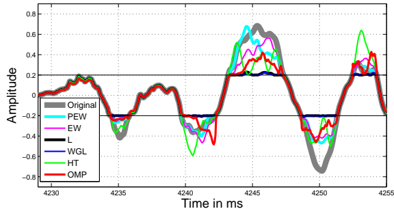
Fig. 2. Declipped music signal using different operators for clip level \theta^{clip} = 0.2 using the Lasso, WGL, EW, PEW, HT, and OMP operators. Neighborhood size for WGL and PEW was 7.
