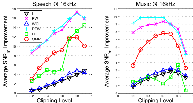
Fig. 4. Average SNR_{miss} for 10 speech (left) and music (right) signals over different clipping levels and operators. Neighborhoods extend 3 and 7 coefficients in time for speech and music signals, respectively.
