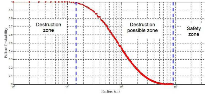
Figure 5: The failure probability and the affected zones resulting from the rupture of TK1.
