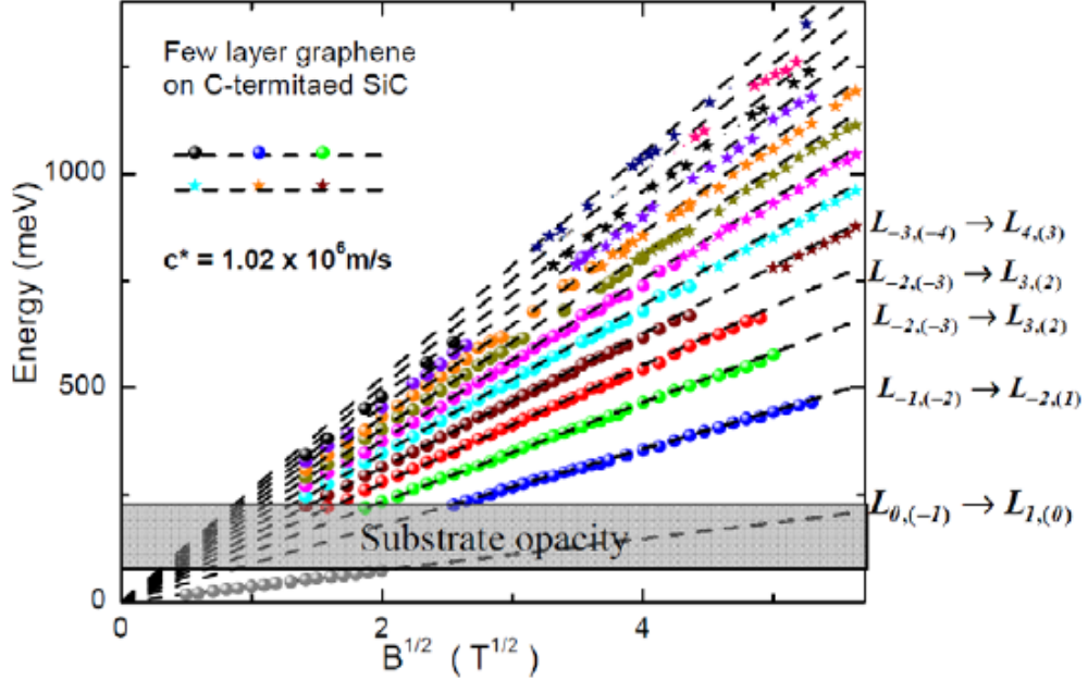
Figure 7: Magnetic field evolution of energetic centres of the magneto-absorption lines observed for few graphene layers on C-terminated surface of SiC. Note the characteristic sequence and almost perfect, linear with square root of magnetic field dependence—an experimental proof for electronic decoupling of layers.
