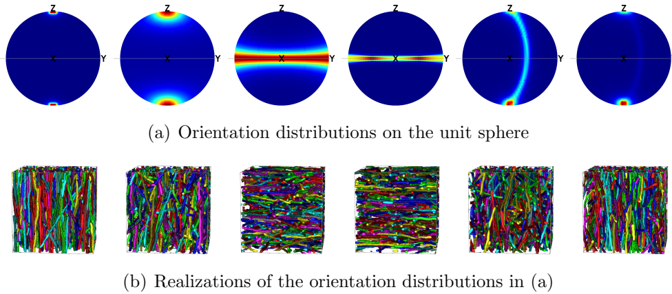
Figure 6: Variety of orientation distributions and their realizations. From left to right: transversely isotropic Z-pref. ( \beta = 0.05 ), Z-pref. ( \beta = 0.3 ), Planar ( \beta = 5 ) and Planar ( \beta = 30 ), and two orthotropic mixed- \beta distributions with q = 0.2 and q = 0.8 .
