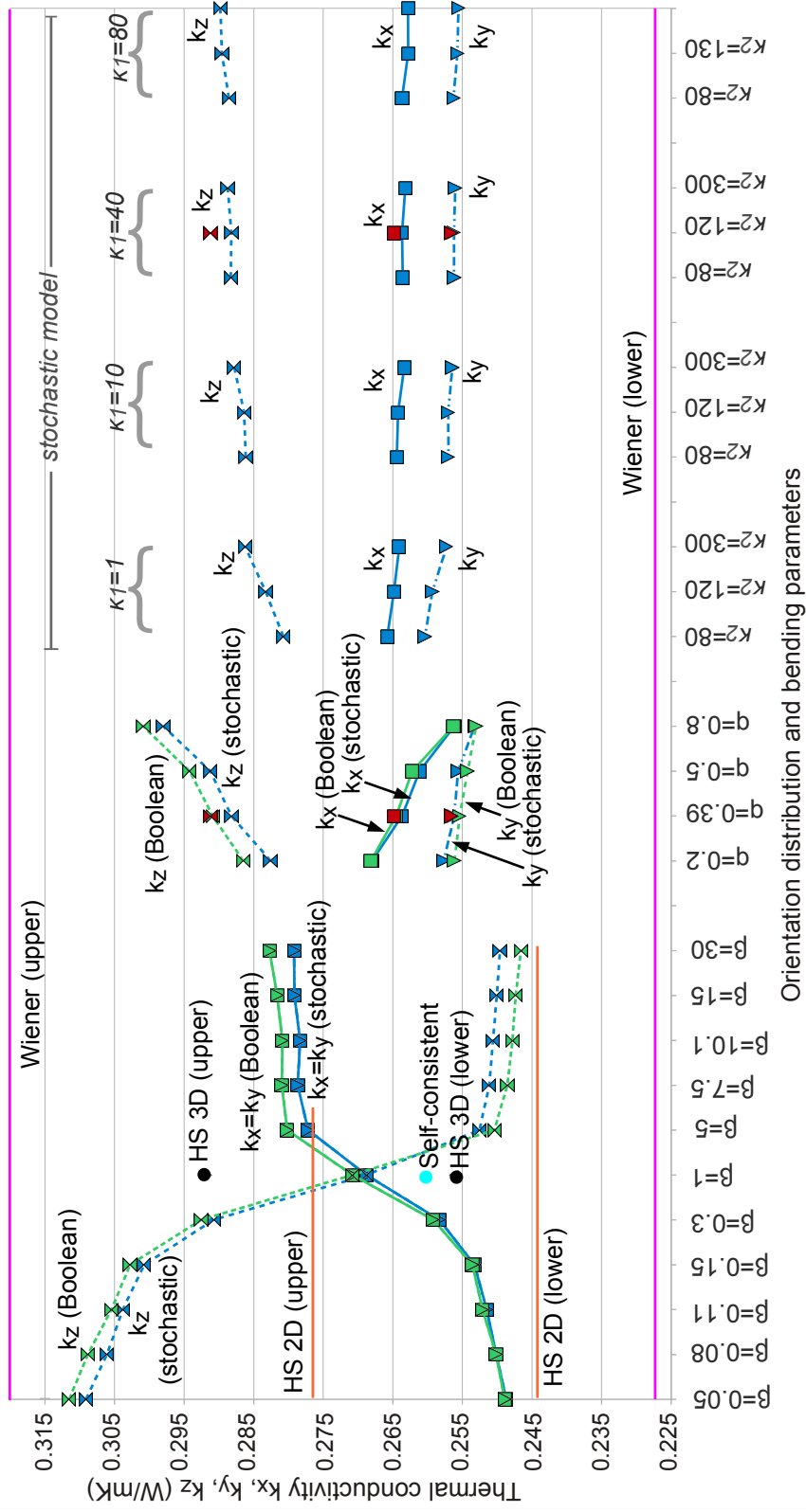
Figure 19: Continuation of figure (17): thermal conductivity components k_x , k_y and k_z . Wiener bounds in magenta.
