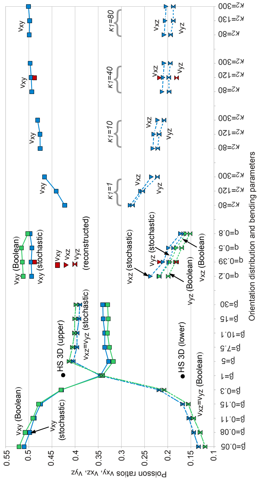
Figure 16: Continuation of figure (15): Poisson ratios \nu_{xy} , \nu_{xz} and \nu_{yz}
