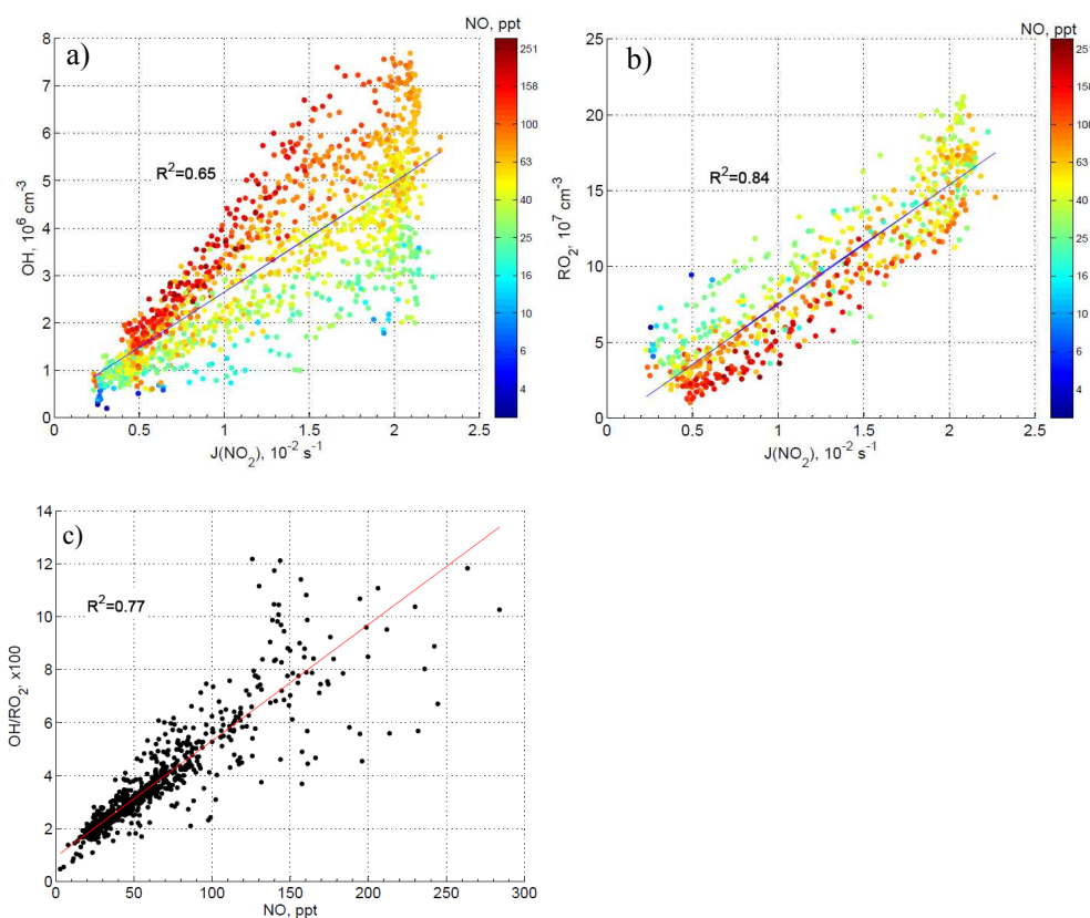
Figure 3. Correlations of [OH] (a) and [RO 2 ] (b) with J(\text{NO}_2) and of [OH] / [RO 2 ] with [NO] (c).
