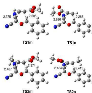
Figure 1 Transition structures involved in the reactions between CY 1'a and methyl propiolate ( 4 ) and methyl but-2-ynoate ( 6 ) (distances are given in Å).
