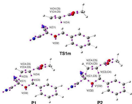
Figure 2 ELF attractors at selected points of the IRC associated with the 32CA reaction between CY 1'a and methyl propiolate ( 4 ).
