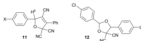
Scheme 1 The different products obtained by reaction of 2,2-dicyano-3-(4-chlorophenyl)oxirane ( 1c ) with 3-phenylpropionitrile ( 10 ).
