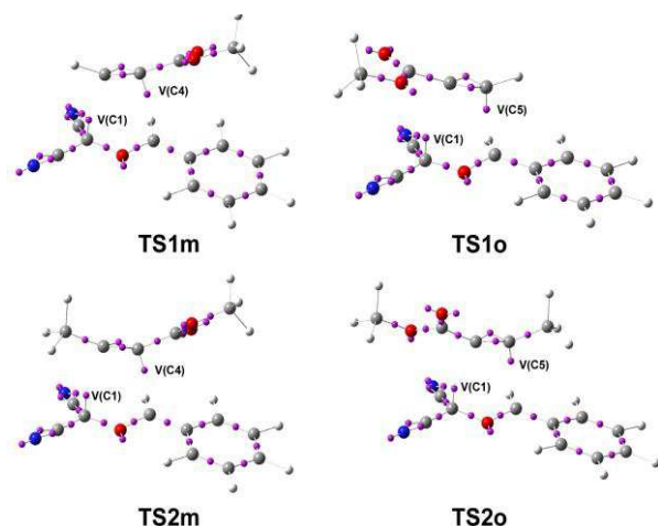
Figure 4 ELF attractors at the TSs involved in the non-polar 32CA reactions between CY 1'a and methyl propiolate ( 4 ) and methyl but-2-ynoate ( 6 ).
