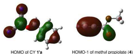
Figure 3 HOMO of CY 1'a and the two electrons of HOMO-1 of methyl propiolate ( 4 ).
